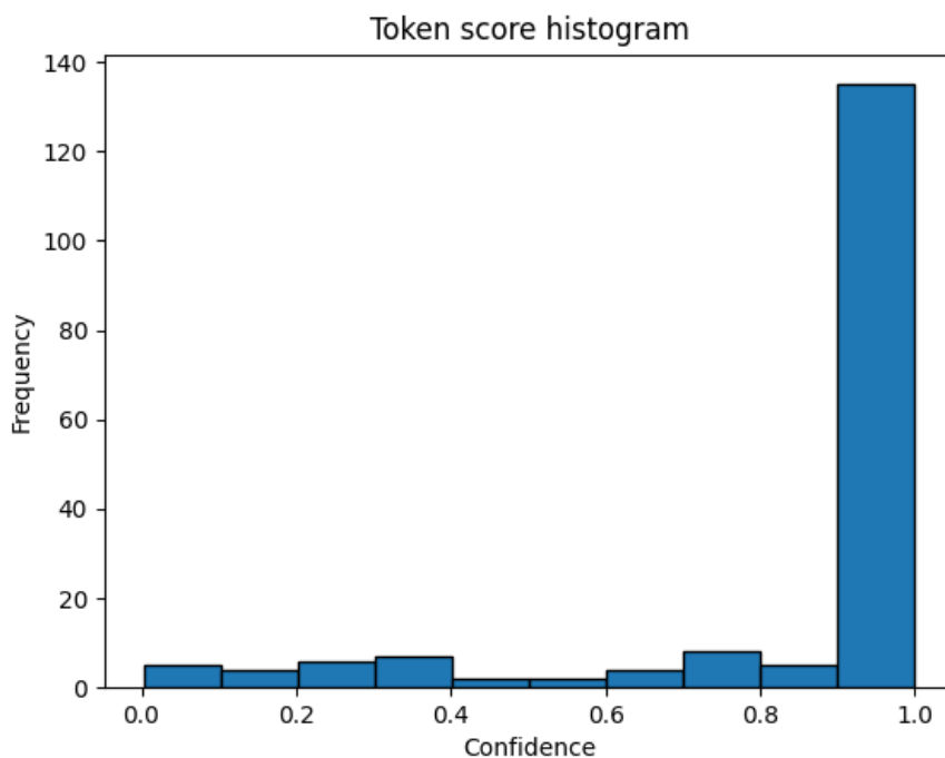
Figure 3.5: Histogram that displays the distribution of the token confidence in the humaneval task 19. The confidence is displayed on the x-axis and the number tokens in each bin are on the y-axis. As we see the model is mostly overconfident in its token selection.
