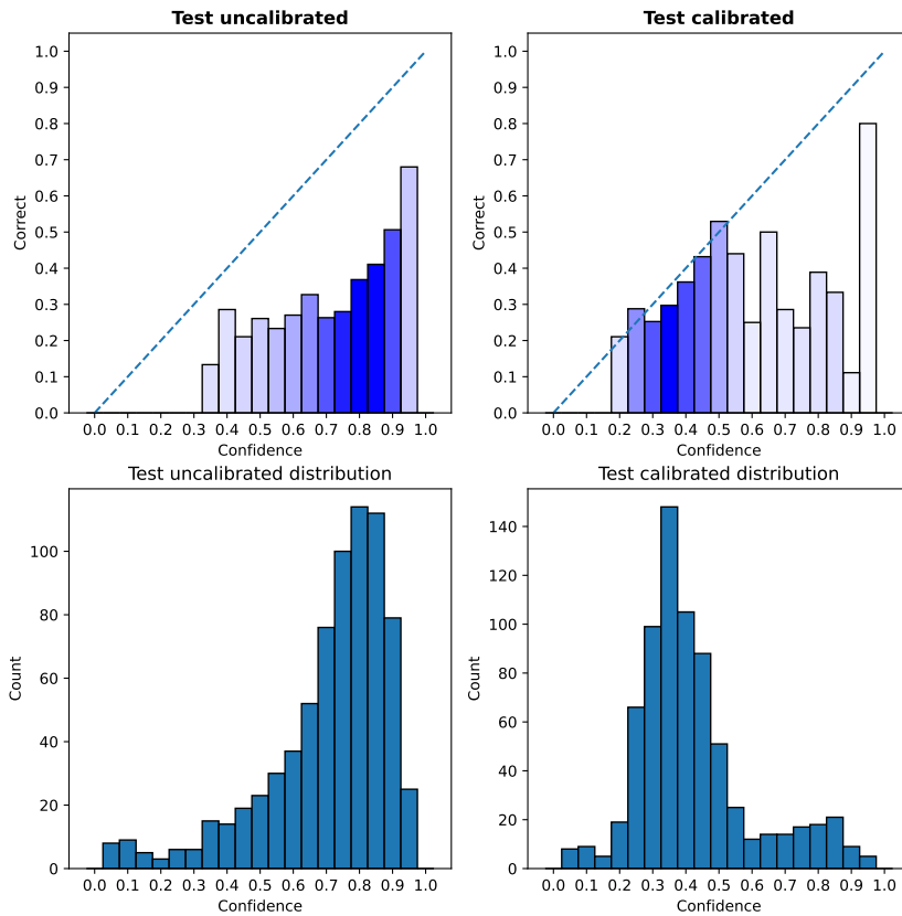
Figure 4.5: Displays the calibration before (left side) and after (right side) the iterative group linear binning approach was used. On the x-axis we got the confidence of the model in the generated code. The y-axis in the upper row displays the correctness in each bin and in the lower row the count of sample in each bin. On the bottom row the distribution our samples are displayed.
