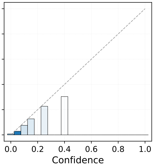
HB
