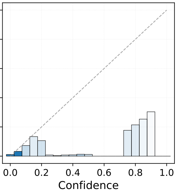
IGHB
