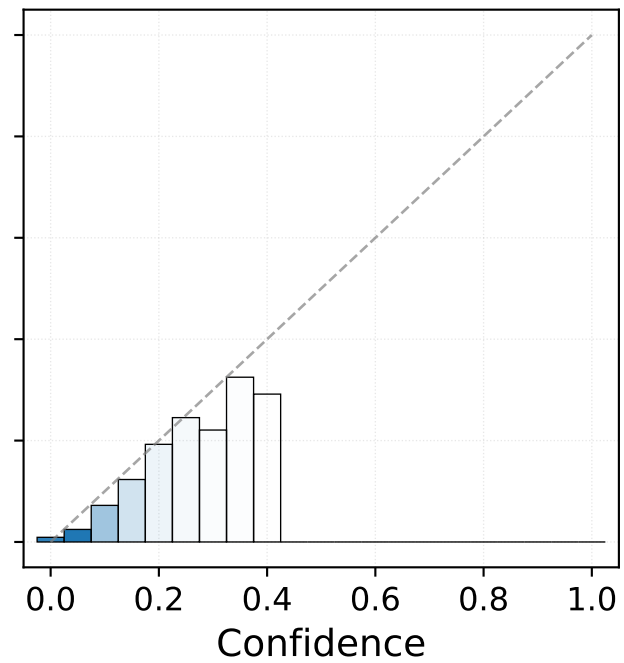
Platt
