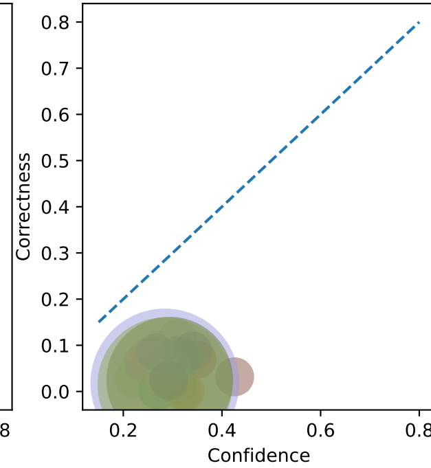
IGHB
