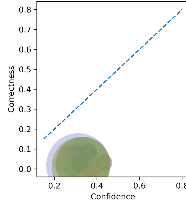
Uncalibrated
