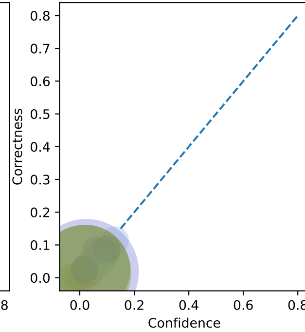
LR
