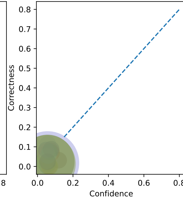
HB
