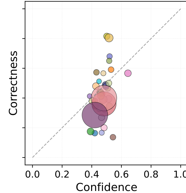
Platt
