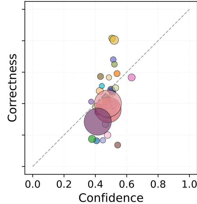
HB
