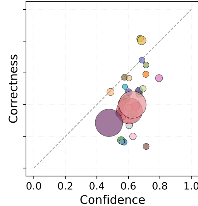
IGHB
