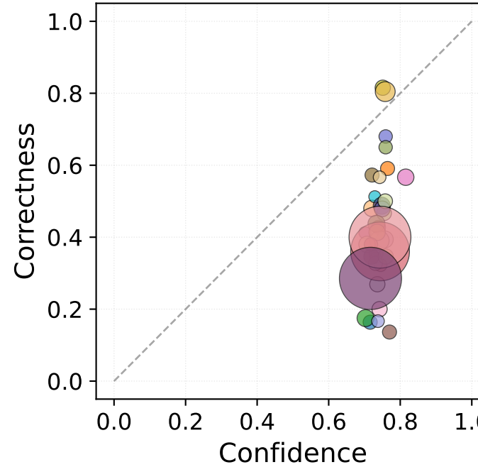
Uncalibrated
