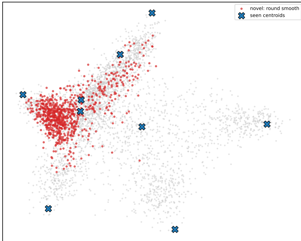
supcon-ft PRE-discovery
