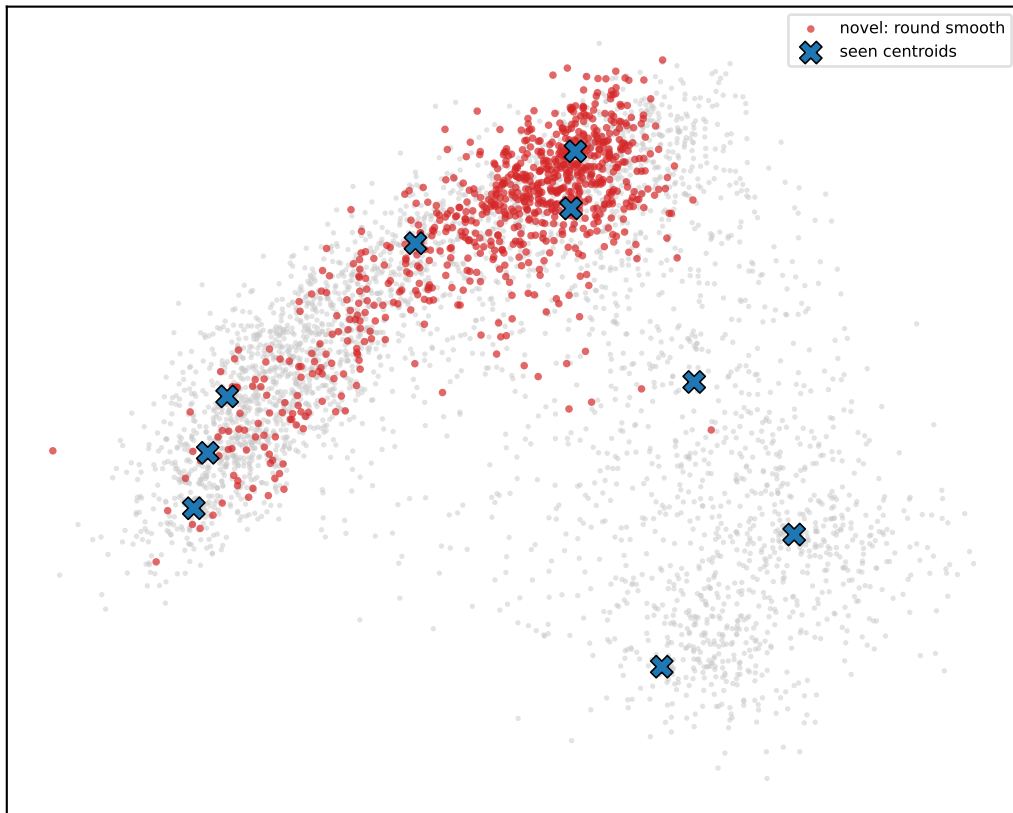
ss-ft PRE-discovery
