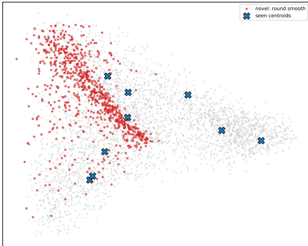
supcon-ft_res PRE-discovery
