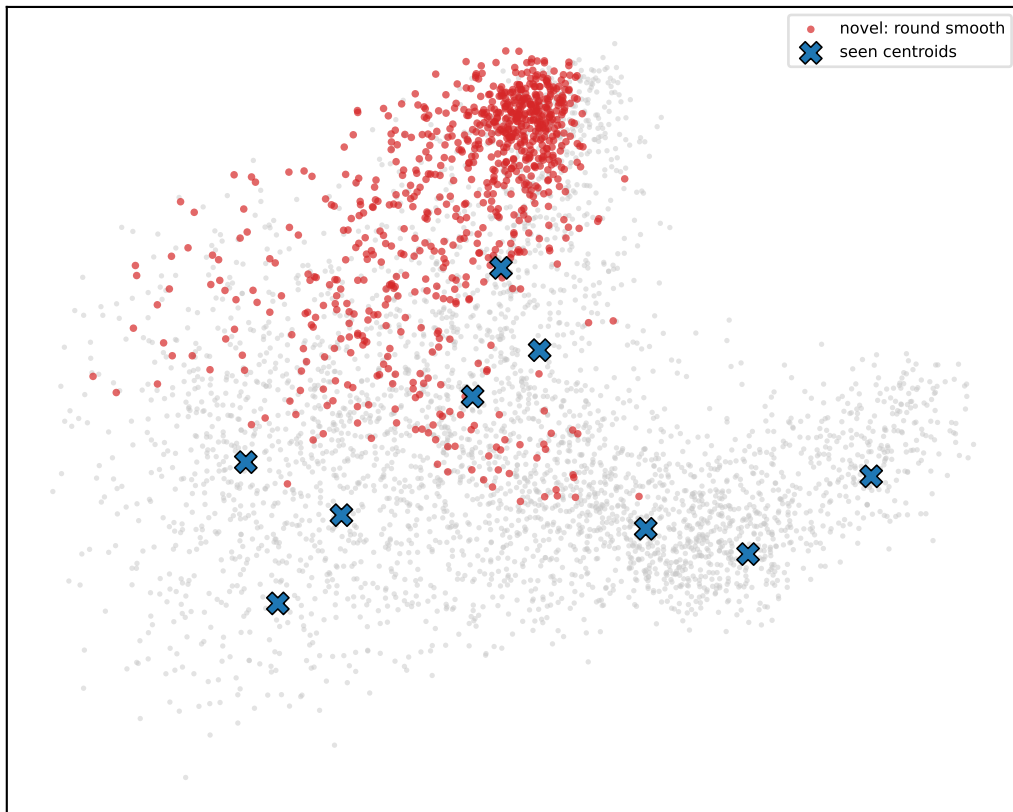
ss-ft_res PRE-discovery
