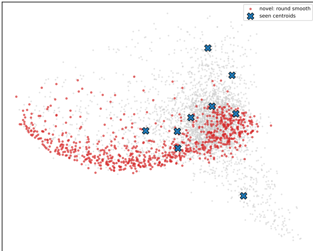
simclr-ft PRE-discovery
