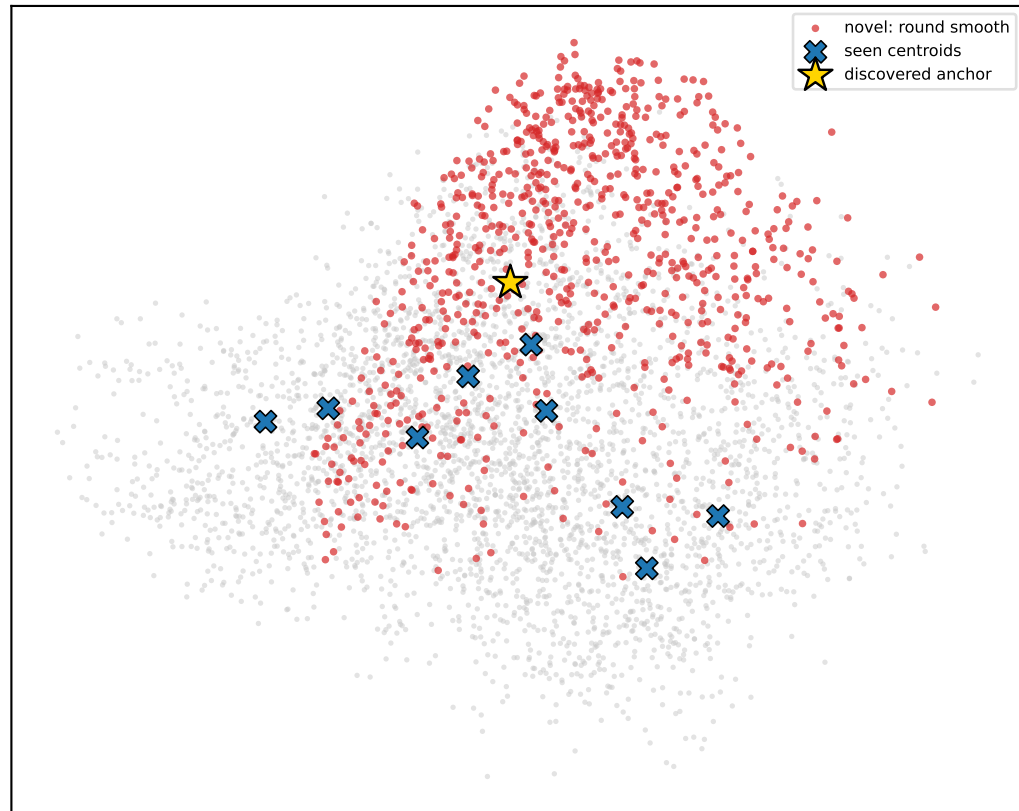
ss-ft_res POST s/ \sqrt{b} (1 anchor)
