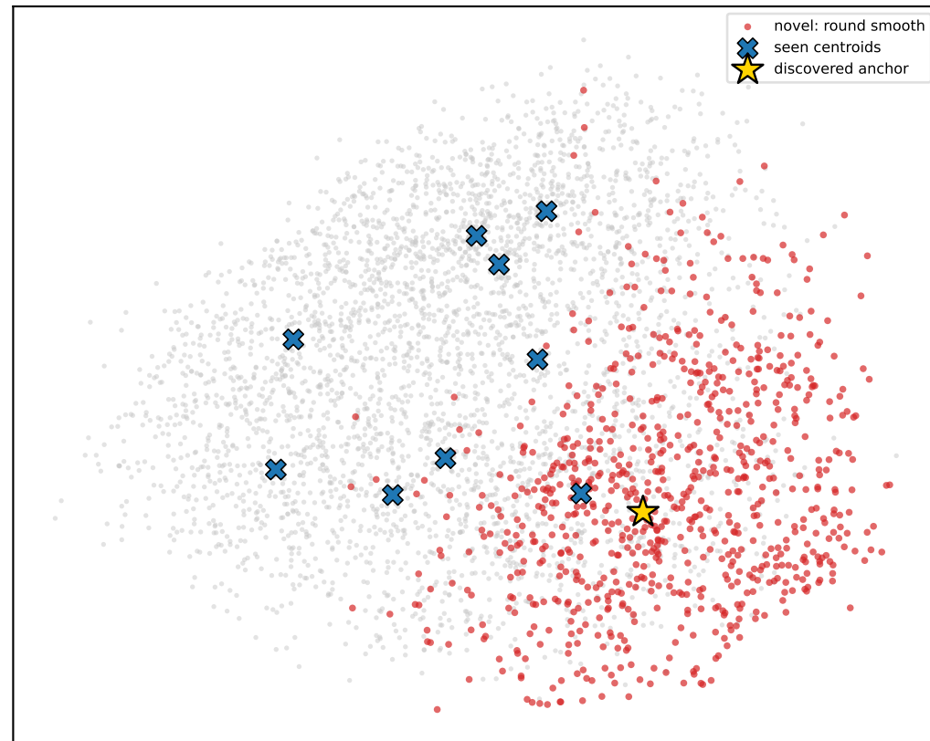
nplm-bil-ft POST s/ \sqrt{b} (1 anchor)
