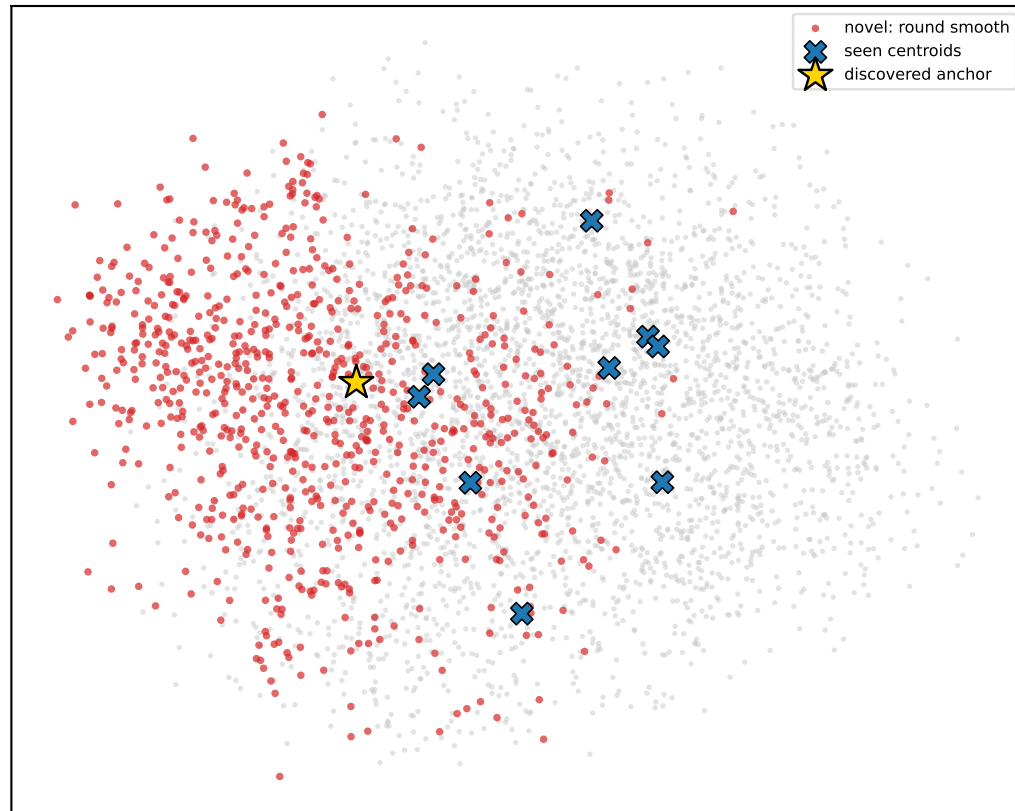
supcon-ft_resnplm POST s/v/b (1 anchor)
