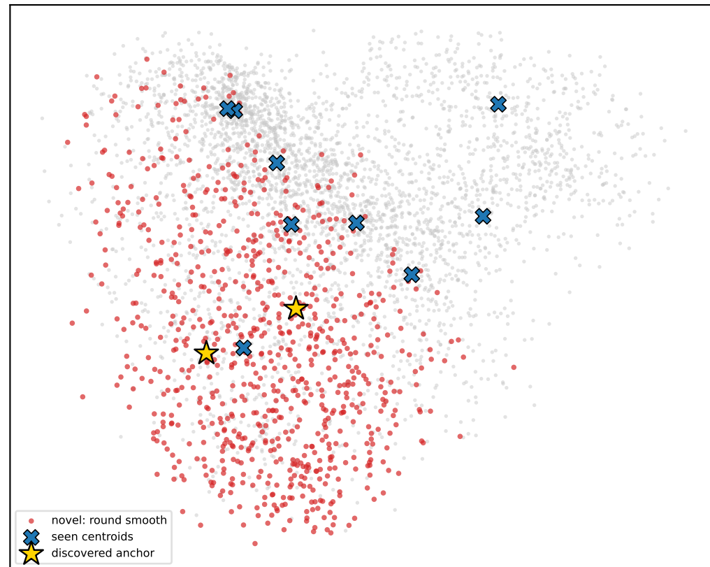
supcon-ft_res POST s/vb (2 anchors)
