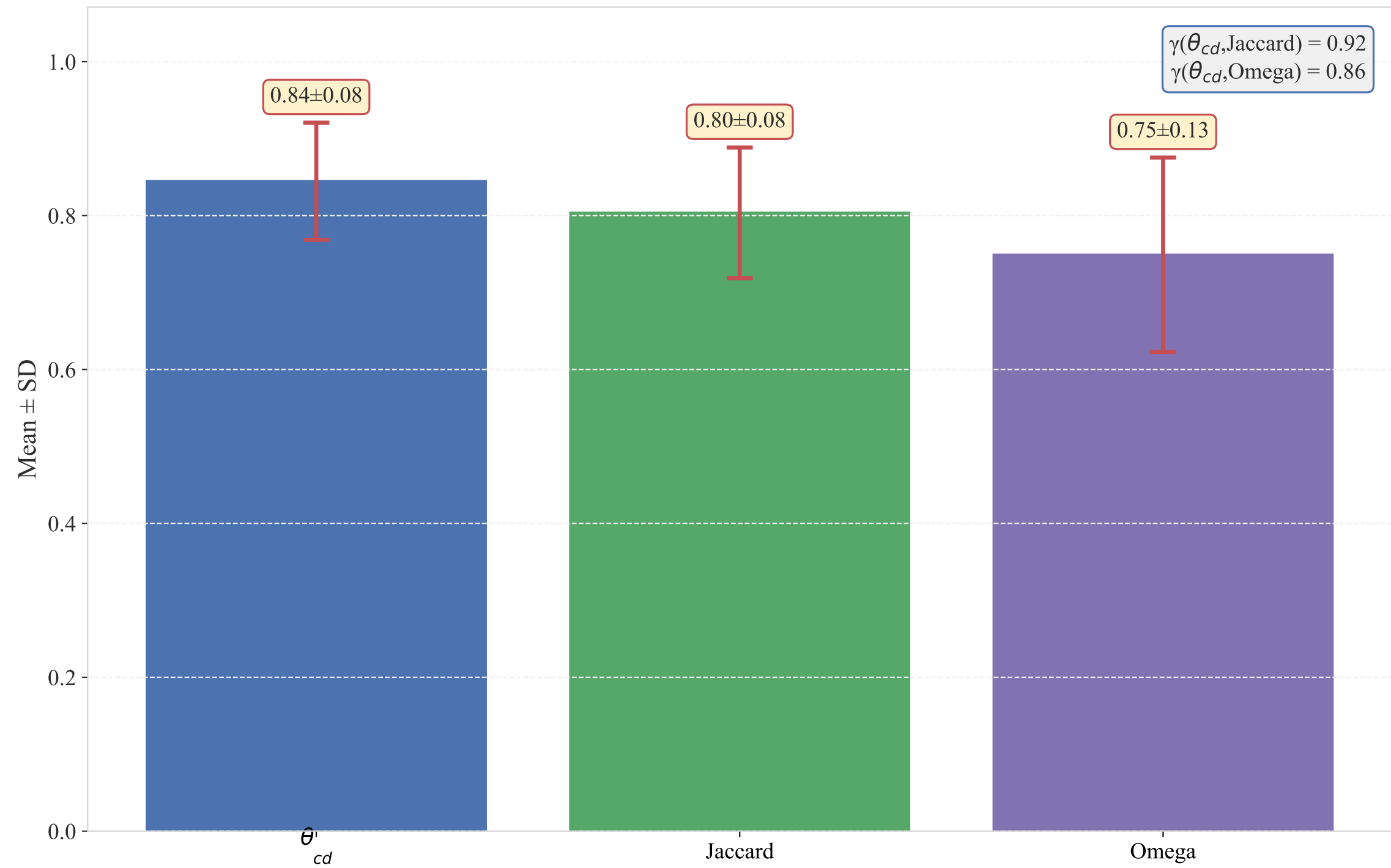
Comparison of Consistency Metrics under 10% Missing
