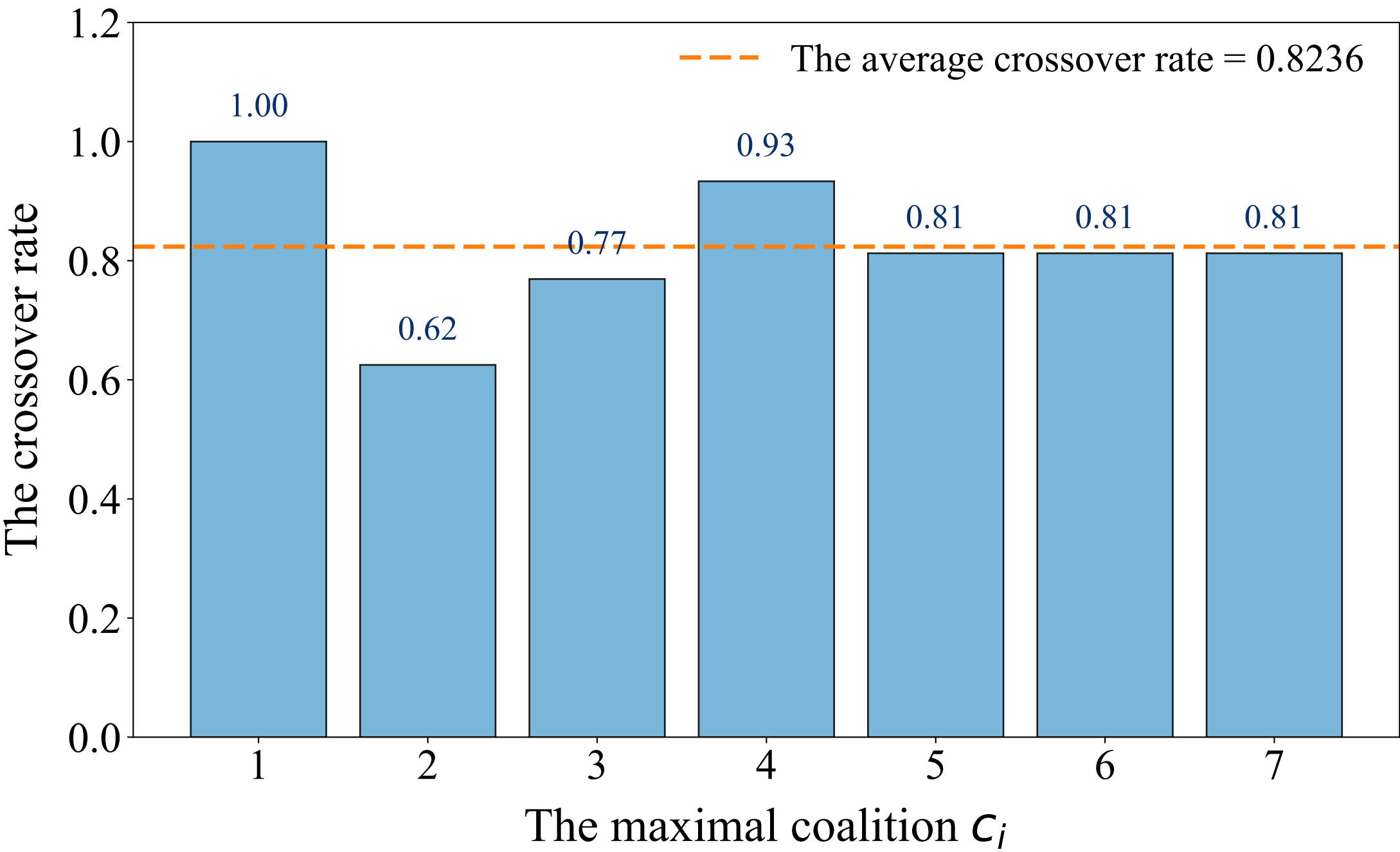
The crossover rate for each maximal coalition C_i
