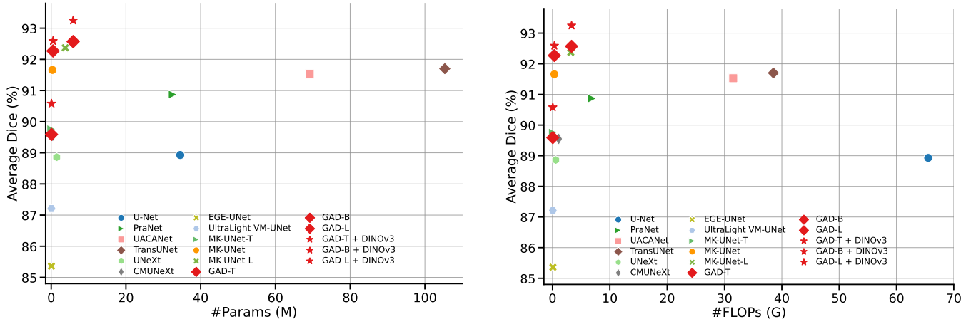
Fig. 1. Accuracy–efficiency comparison across PH 2 , ISIC2018, CVC-ClinicDB, and CVC-ColonDB. The vertical axis reports the macro-average Dice score over the four datasets, while the horizontal axes show student-side parameters and FLOPs. Compared with existing lightweight segmentation networks, GAD-MambaUNet achieves a more favorable balance between segmentation accuracy and deployment cost. The DINOv3 teacher is used only during training and is excluded from deployment cost.
