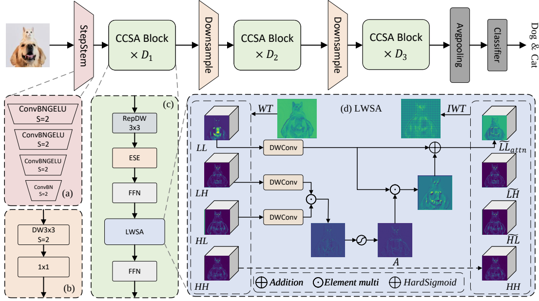
Figure 5: Overall architecture of WCANet and its main components. (a) StepStem; (b) downsampling block; (c) CCSA block; and (d) Learnable Wavelet Spatial Attention (LWSA).
