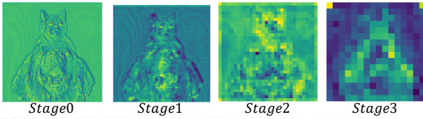
Figure 3: Feature map evolution from Stage 0 to Stage 3 of WCANet, illustrating the progressive transformation of feature representations across network depth.
