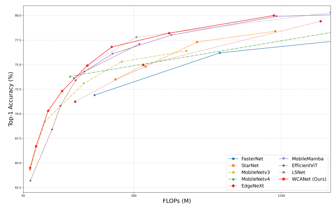
Figure 1: Accuracy-computation comparison between WCANet and representative lightweight vision models on ImageNet-1K. The figure illustrates the accuracy-efficiency trade-off under different computational budgets.
