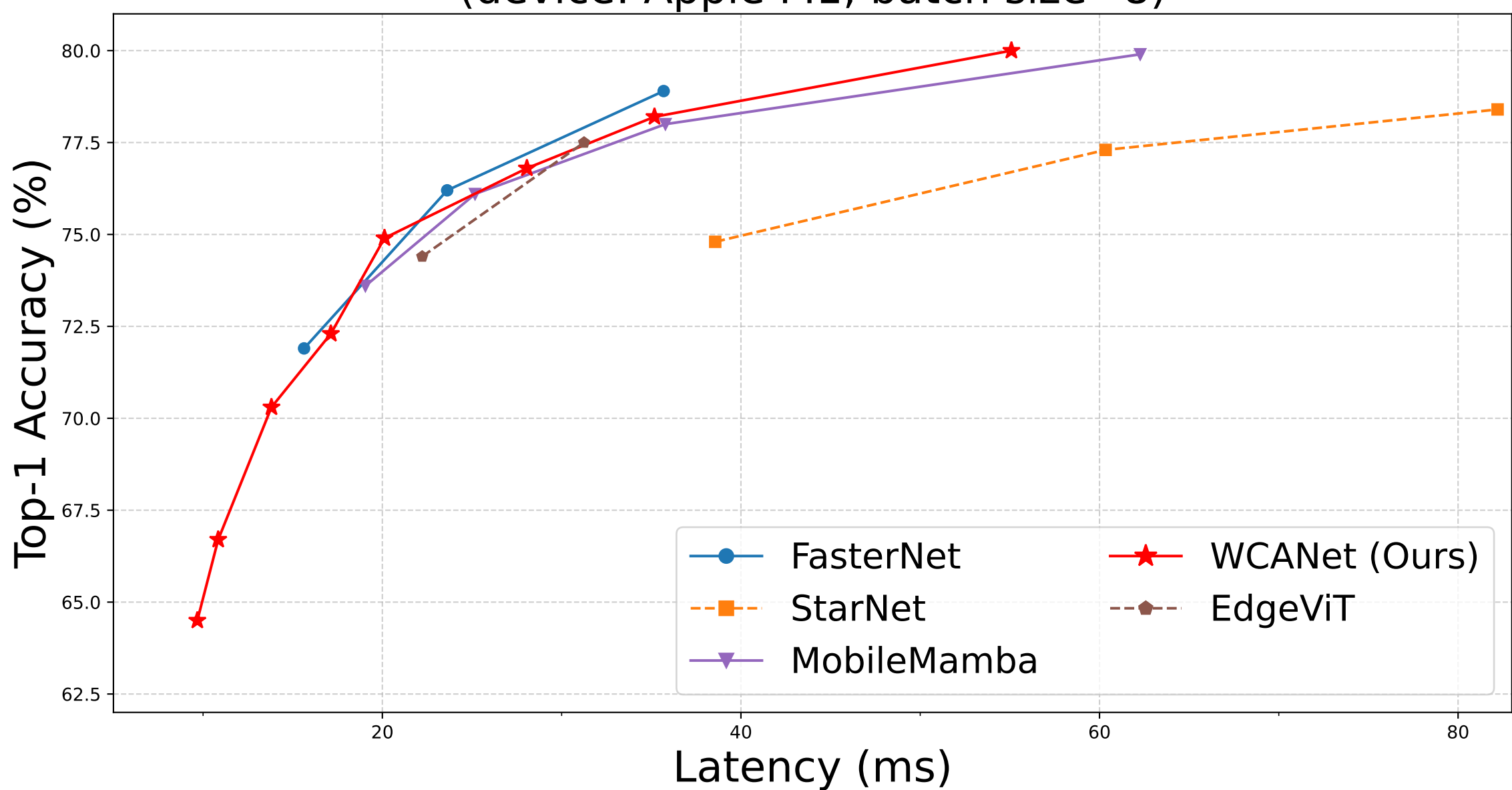
Latency vs Top-1 Accuracy (device: Apple M1, batch size=8)
