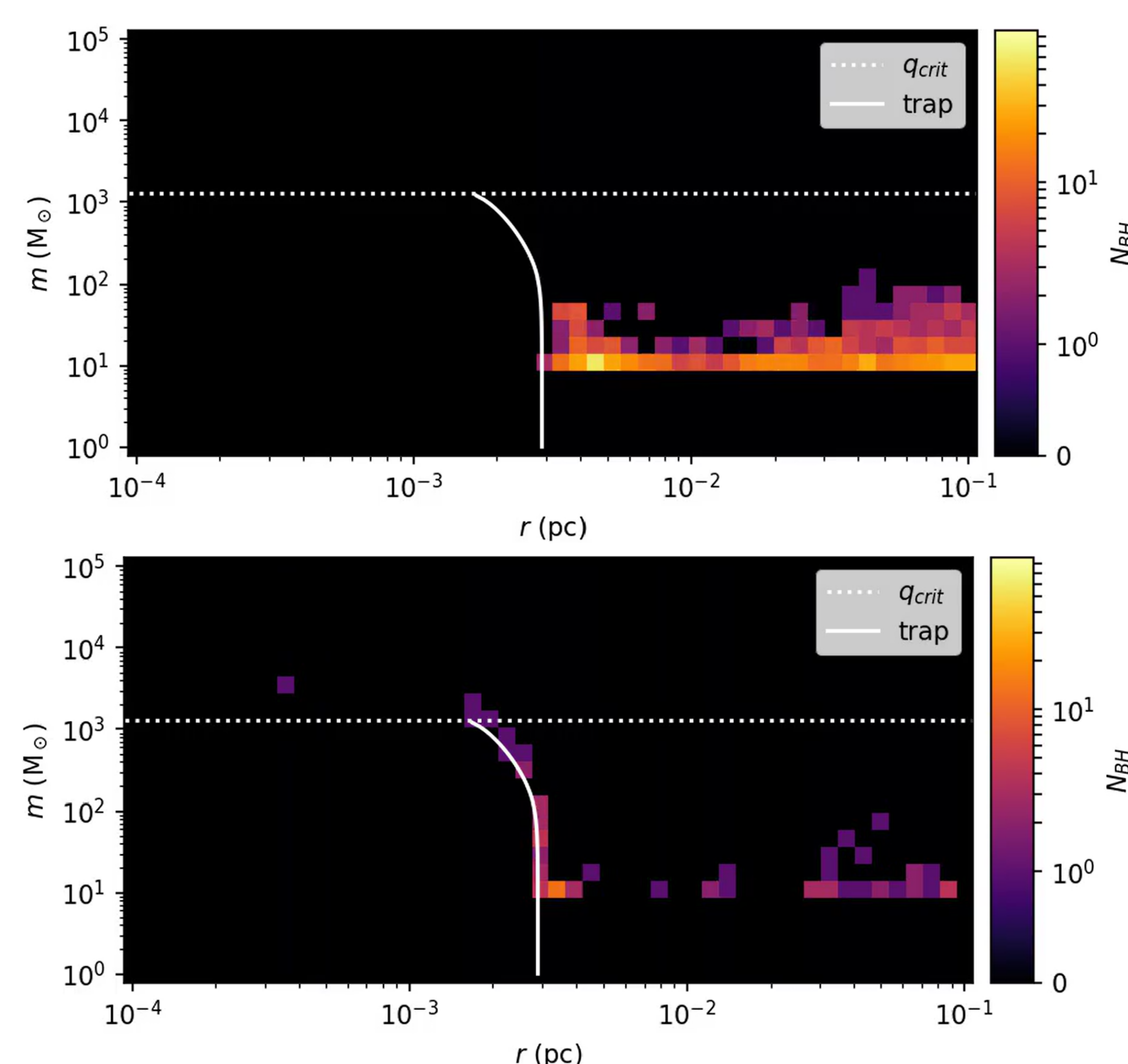
Figure 2: Two snapshots of a histogram of the simulated BHs across the m - r space (see Section 6), one shortly after the beginning (top panel) and one at a later time (bottom panel). Solid white line: trap position for each BH mass, solved from equation (1). Dotted white line: critical mass ratio q = m/M_{\text{SMBH}} where IMBHs decouple from the trap.
