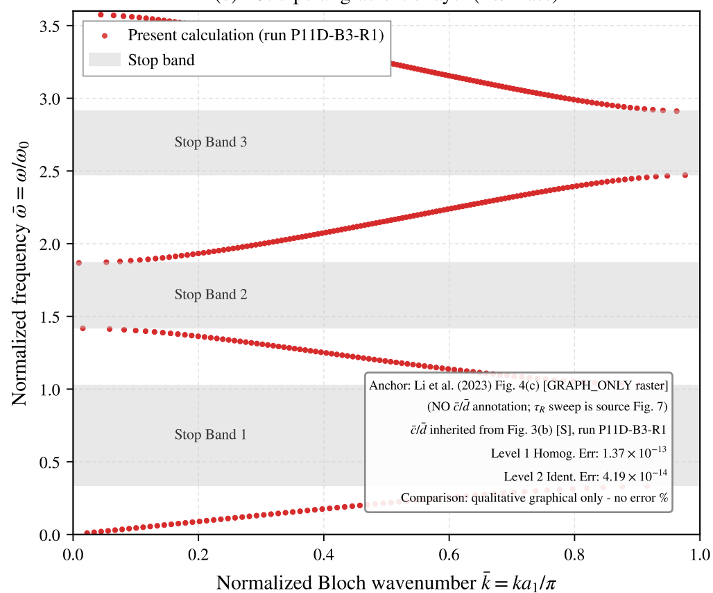
(b) B3: dipolar gradient bilayer (Pb/Brass)
