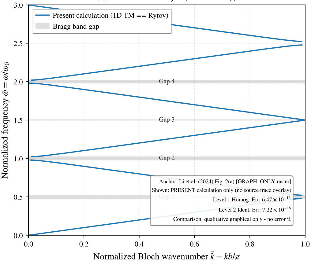
(a) B1: classical bilayer (AlN/BaTiO 3 )
