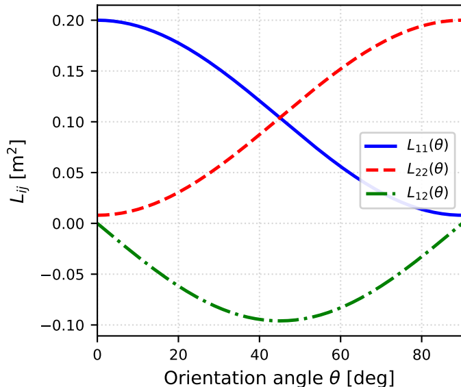
(b) Tensor Components \mathbf{L}(\theta) (AR = 5)
