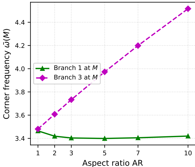
(b) Frequencies at M vs AR
