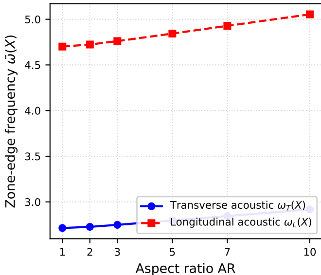
(a) Acoustic Frequencies at X vs AR
