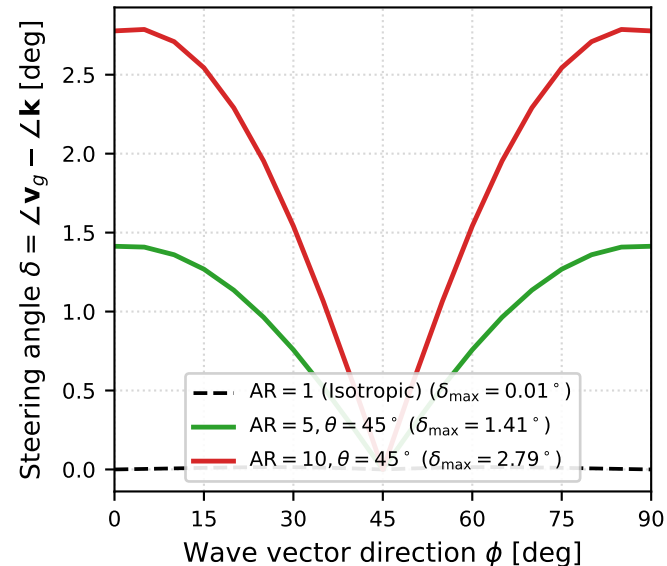
(a) Energy Deviation Angle
