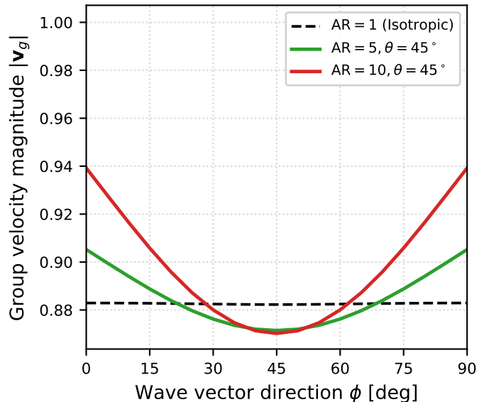
(b) Group Velocity Anisotropy
