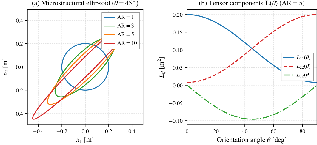
Figure 1: (a) Schematic of the microstructural averaging ellipsoid at orientation \theta = 45^\circ for aspect ratios AR \in \{1, 3, 5, 10\} under volume-equivalent scaling ( l_{\text{iso}} = 0.20 \text{ m} ). (b) Evolution of second-moment length tensor components L_{11}, L_{22}, L_{12} as functions of orientation angle \theta for AR = 5 , verifying negative off-diagonal coupling L_{12}(45^\circ) = -0.096 \text{ m}^2 under locked passive rotation.
