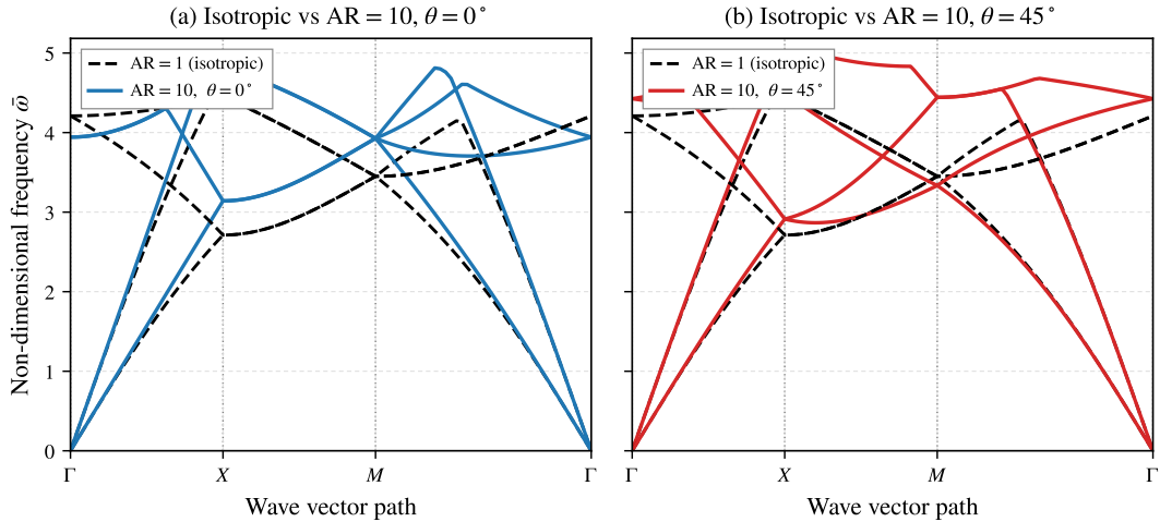
Figure 6: Bloch band structure along \Gamma -X-M- \Gamma for Case H ( L = 1.0 m, \rho = 1.0 kg/m 3 , \mu = 1.0 Pa, \nu = 0.25 , l_{\text{iso}} = 0.20 m, \ell_i = 0.20 m). (a) Isotropic baseline (AR = 1) versus anisotropic microstructure aligned with the lattice (AR = 10, \theta = 0^\circ ). (b) Isotropic baseline (AR = 1) versus diagonal anisotropic microstructure (AR = 10, \theta = 45^\circ ), highlighting the opening of directional stop band \Delta_{GX} = +0.0043 along \Gamma -X while strictly preserving the absence of complete omnidirectional band gaps ( \Delta_{\text{complete}} \leq -0.3235 ).
