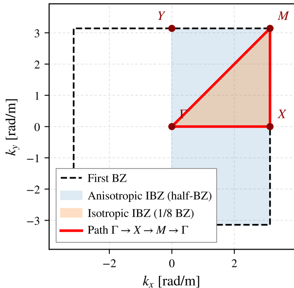
(b) Reciprocal space &amp; symmetry path
