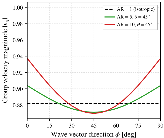
(b) Group velocity magnitude at \bar{k} = 0.5
