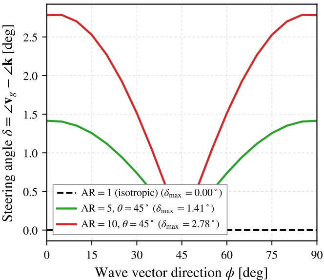
(a) Steering deviation \delta(\phi) at \bar{k} = 0.5
