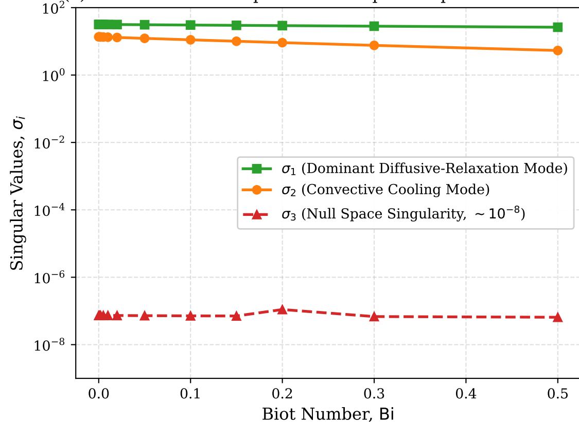
(a) 3-Parameter SVD Spectrum: Complete Separation of Modes
