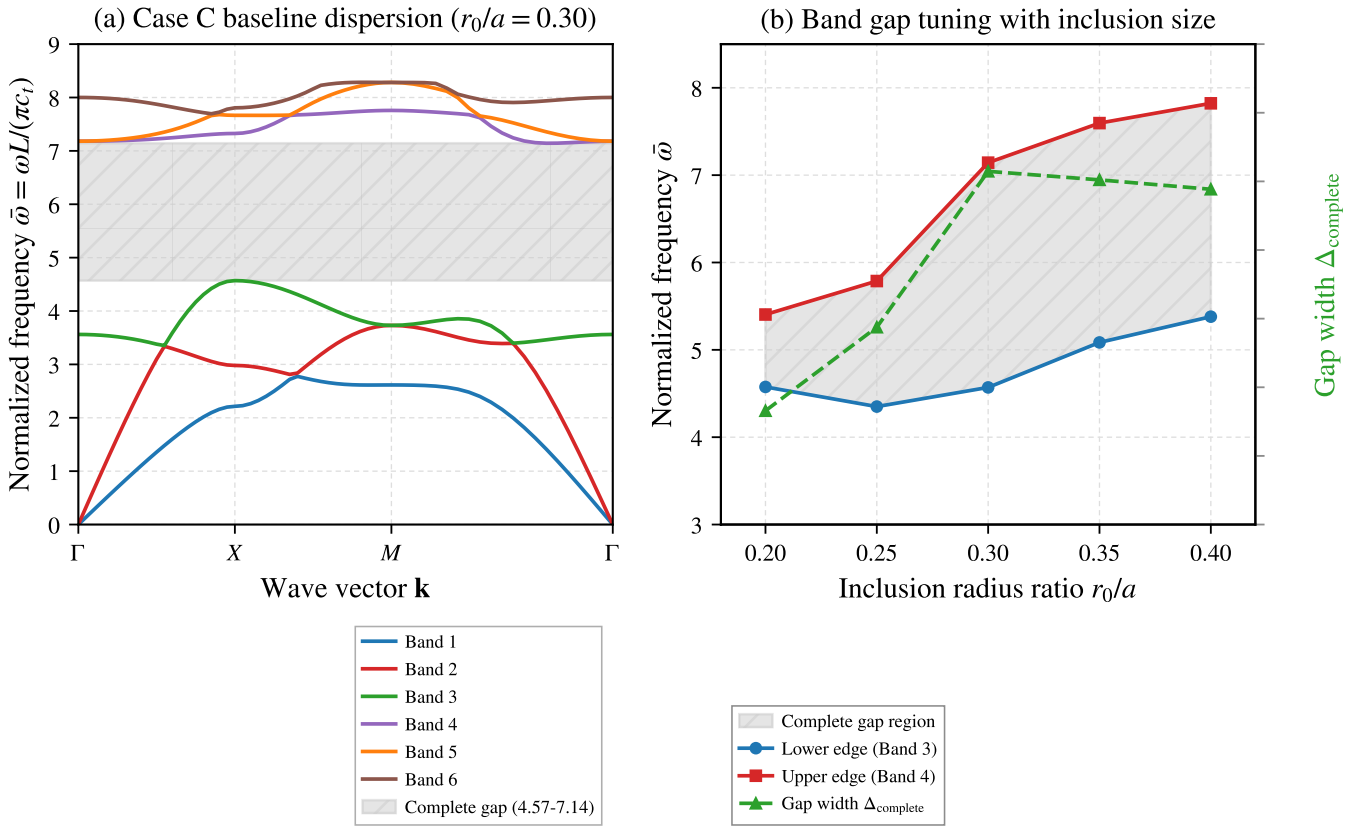
Figure 12: Case-C complete-gap formation and radius dependence. (a) Bands along \Gamma - X - M - \Gamma for r_0/L = 0.30 , with the 4 \times 4 -mesh gap between Bands 3 and 4. (b) Complete-gap width versus r_0/a at the same mesh; the r_0/a = 0.30 result is not mesh-converged.
