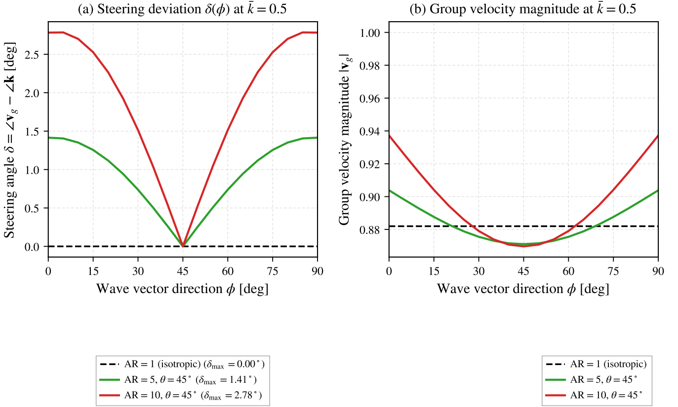
Figure 10: Acoustic-branch group-velocity steering on |\mathbf{k}| = 0.5 at \theta = 45^\circ . (a) Angular deviation for AR = 1, 5, 10, with peak values 0^\circ , 1.4146^\circ , and 2.7846^\circ . (b) Directional variation of group-velocity magnitude.
