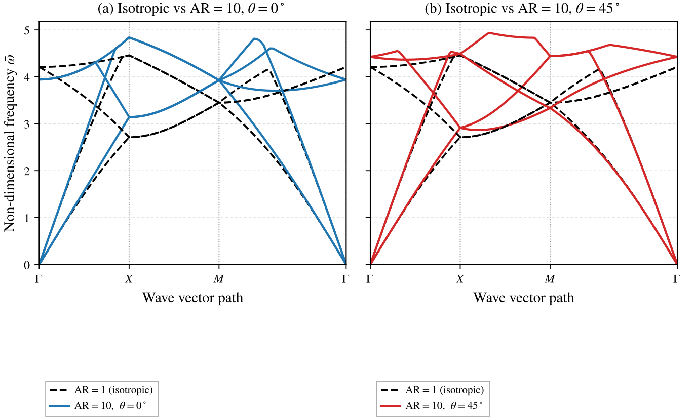
Figure 5: Case-H Bloch bands along \Gamma -X-M- \Gamma . (a) Isotropic reference (AR = 1) and aligned anisotropy (AR = 10, \theta = 0^\circ ). (b) Isotropic reference and diagonal anisotropy (AR = 10, \theta = 45^\circ ), which opens a \Gamma -X stop band but no complete gap.
