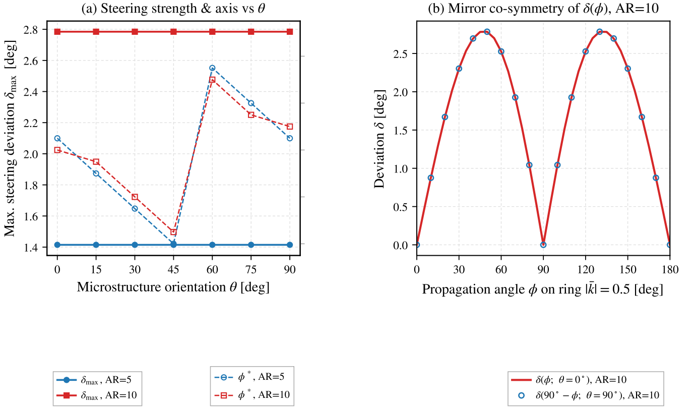
Figure 11: Orientation dependence of steering on |\mathbf{k}| = 0.5 . (a) Peak deviation \delta_{\max} and principal direction \phi^* for AR = 5, 10; the peak angular deviation is invariant over the sampled orientations, while the lobe direction follows the rotated tensor axes on the 5^\circ ring grid. (b) The \theta = 0^\circ and 90^\circ deviation fields at AR = 10 exhibit mirror co-symmetry.
