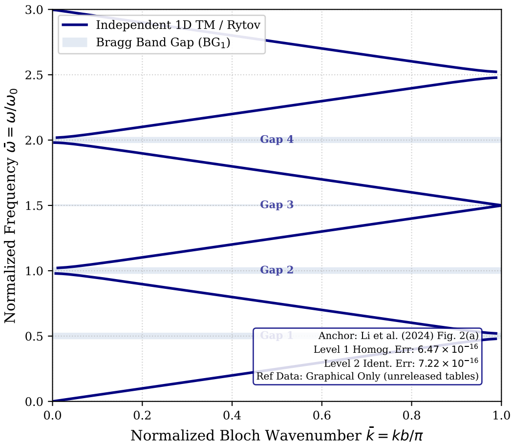
(a) Benchmark B1: Classical Bilayer (AlN/BaTiO 3 )
