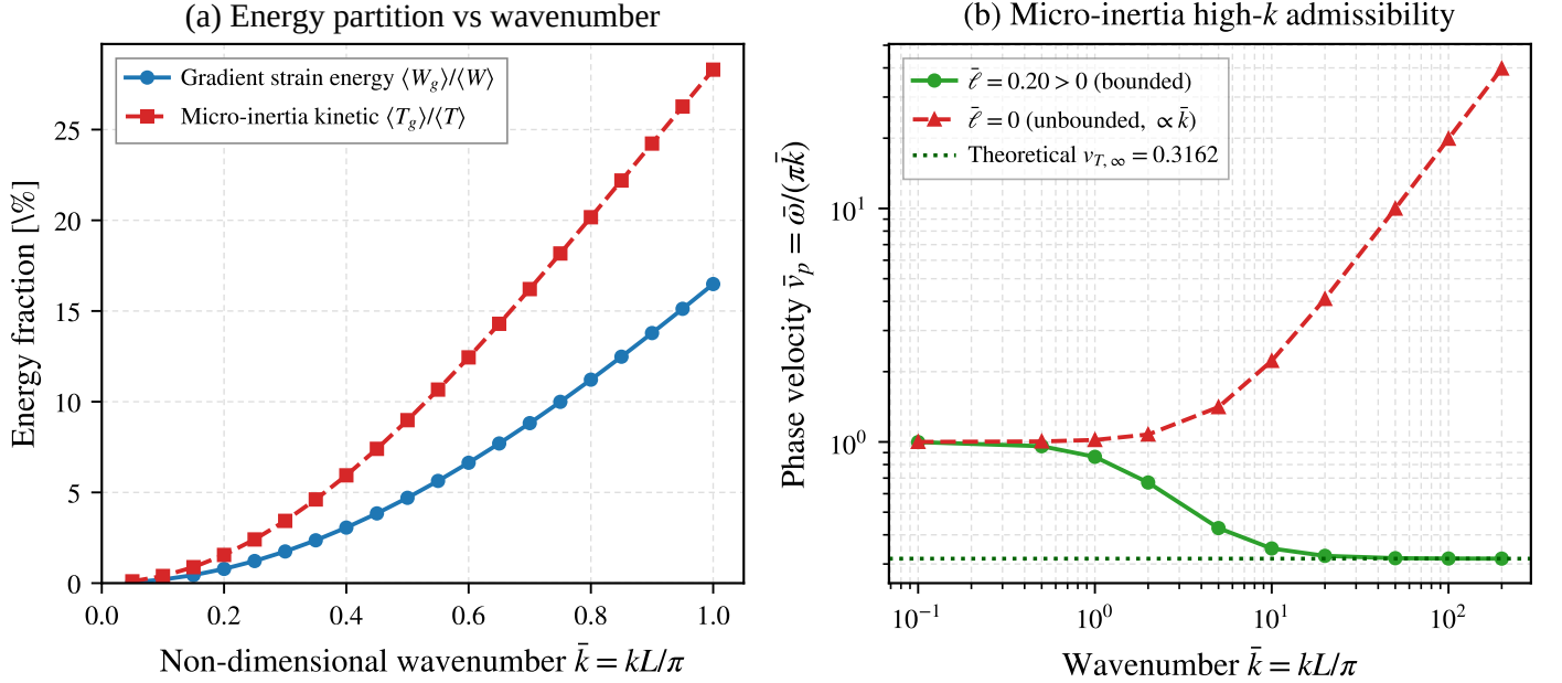
Figure 13: (a) Gradient-energy fraction W_g/W versus wavenumber. (b) Transverse-branch phase velocity with and without gradient micro-inertia; the finite high-wavenumber limit is specific to the shear branch analyzed here.
