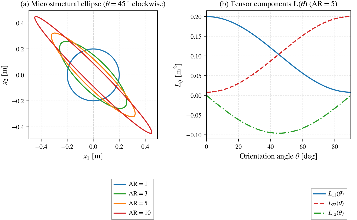
Figure 1: (a) Area-preserving averaging ellipses at \theta = 45^\circ for \text{AR} = 1, 3, 5, 10 , with positive orientation measured clockwise. (b) Length-tensor components versus orientation for \text{AR} = 5 , including L_{12}(45^\circ) = -0.096 \text{ m}^2 under the same passive-rotation convention.
