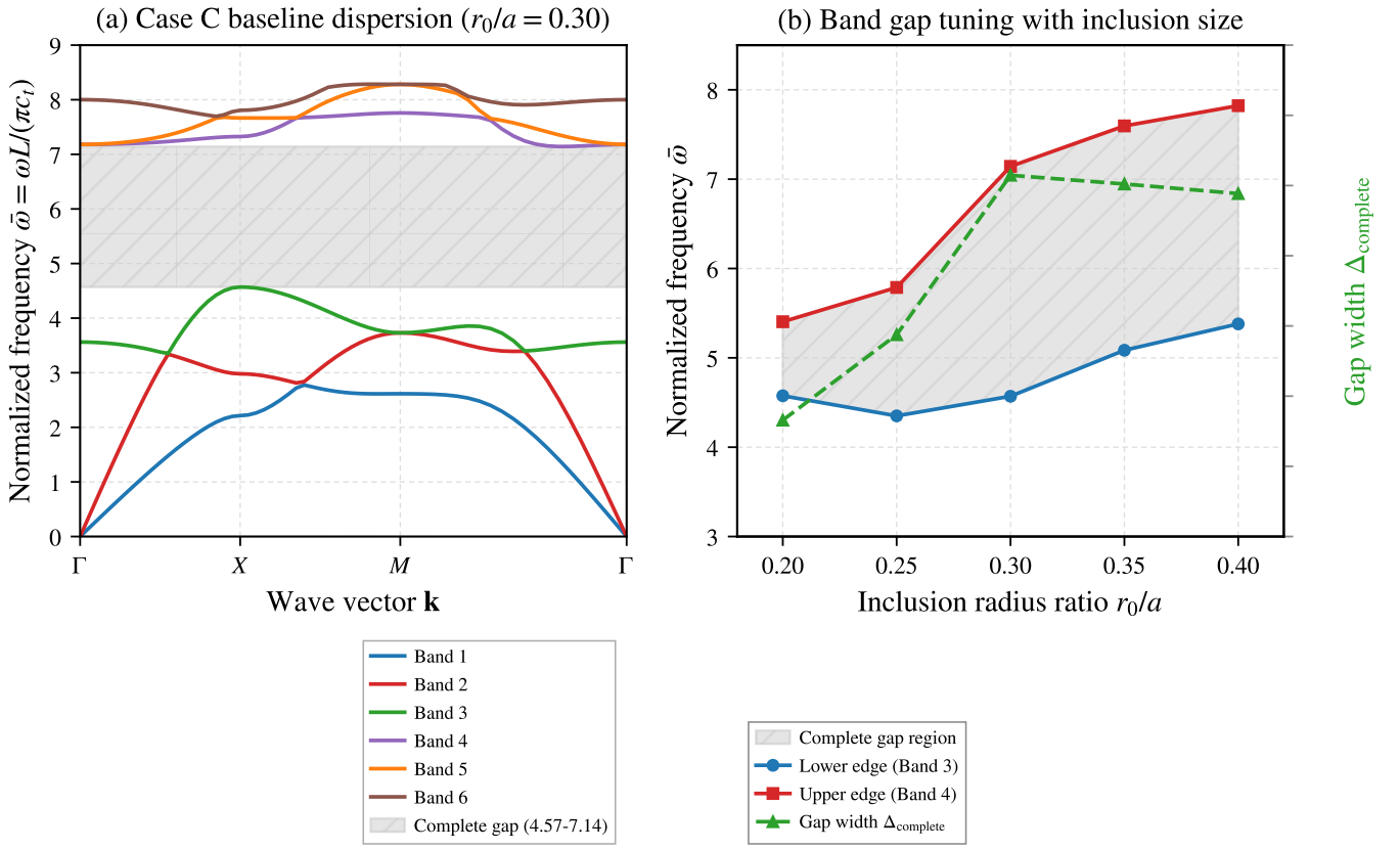
Figure 12: Case-C complete-gap formation and radius dependence. (a) Bands along \Gamma-X-M-\Gamma for r_0/L = 0.30 , with the 4 \times 4 -mesh gap between Bands 3 and 4. (b) Complete-gap width versus r_0/a at the same mesh; the r_0/a = 0.30 result is not mesh-converged.
