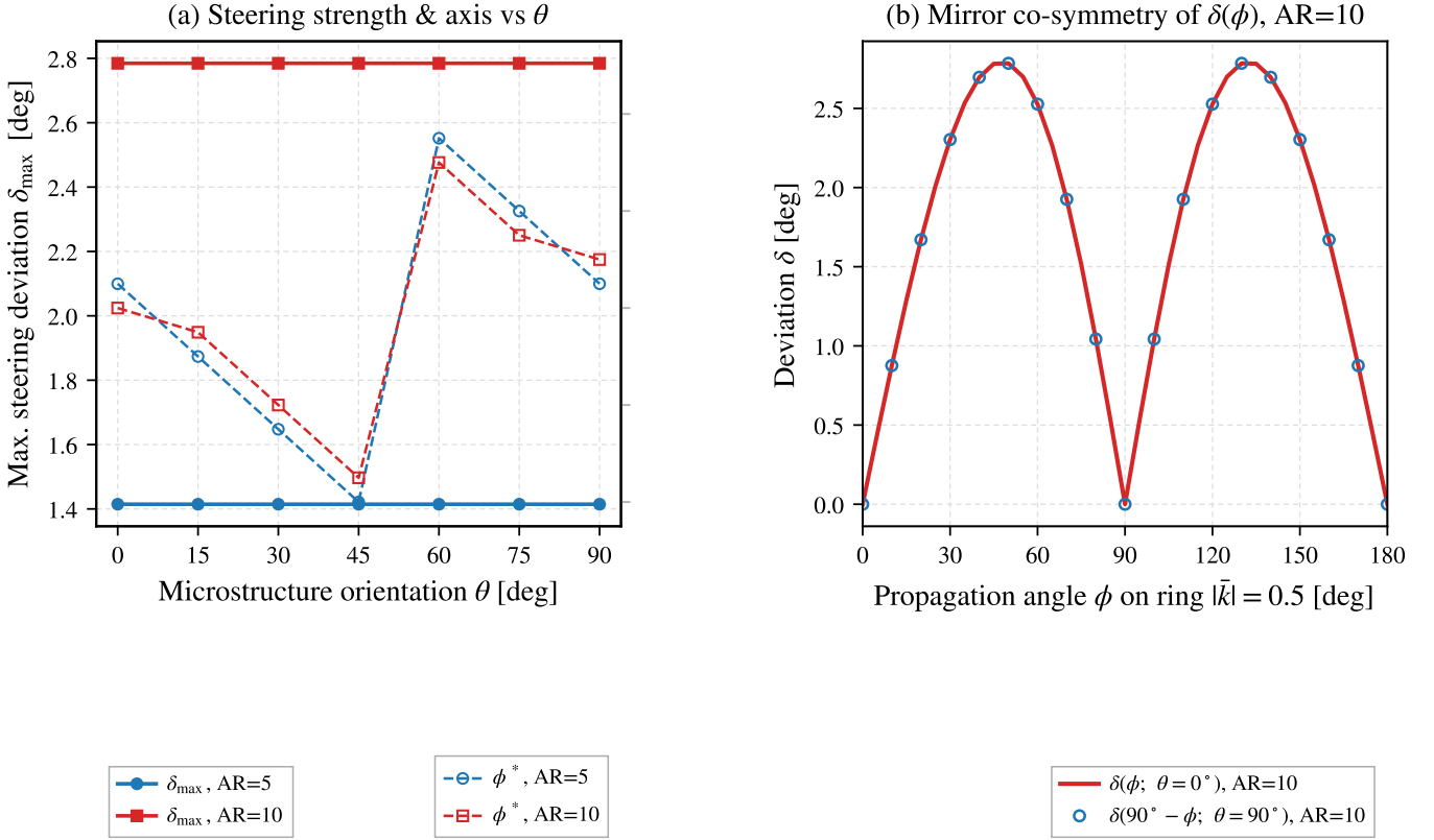
Figure 11: Orientation dependence of steering on |\mathbf{k}| = 0.5 . (a) Peak deviation \delta_{\max} and principal direction \phi^* for \text{AR} = 5, 10 ; the peak angular deviation is invariant over the sampled orientations, while the lobe direction follows the rotated tensor axes on the 5^\circ ring grid. (b) The \theta = 0^\circ and 90^\circ deviation fields at \text{AR} = 10 exhibit mirror co-symmetry.
