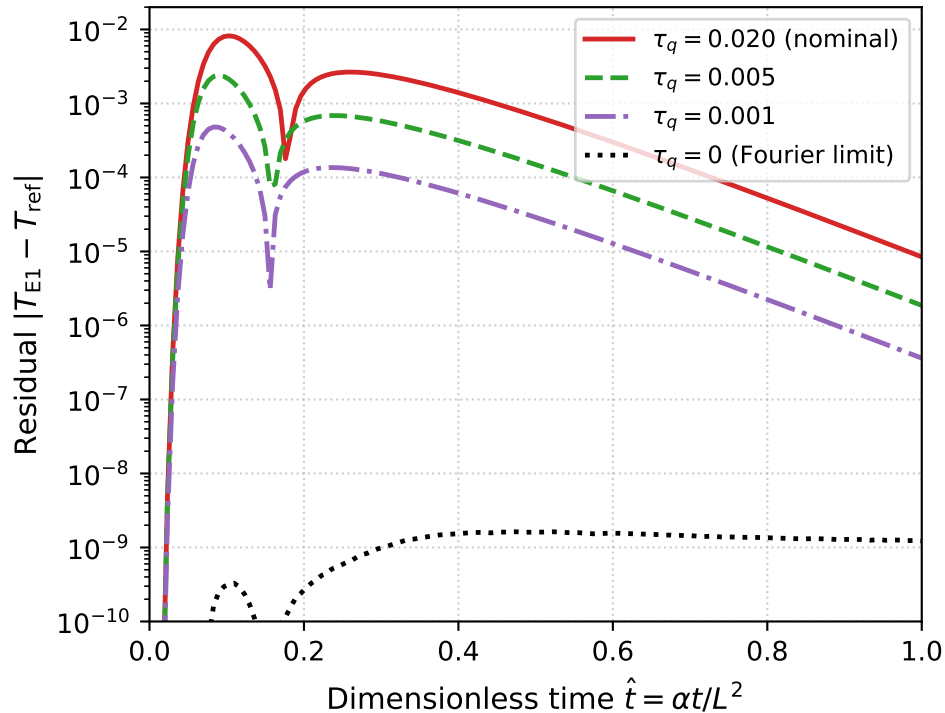
(b) Fourier-Limit Convergence ( \epsilon_\lambda = 0.05 )
