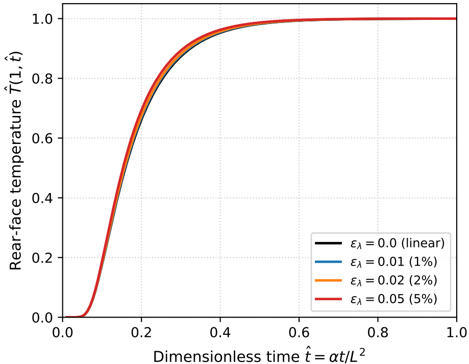
(a) Rear-Face Thermograms
