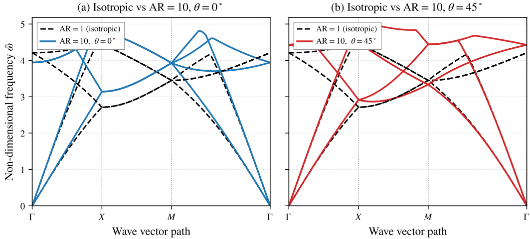
Figure 6: Bloch band structure along \Gamma - X - M - \Gamma for Case H ( L = 1.0 m, \rho = 1.0 kg/m 3 , \mu = 1.0 Pa, \nu = 0.25 , l_{\text{iso}} = 0.20 m, \ell_i = 0.20 m). (a) Isotropic baseline ( AR = 1 ) versus anisotropic microstructure aligned with the lattice ( AR = 10, \theta = 0^\circ ). (b) Isotropic baseline ( AR = 1 ) versus diagonal anisotropic microstructure ( AR = 10, \theta = 45^\circ ), highlighting the opening of directional stop band \Delta_{GX} = +0.0043 along \Gamma - X while strictly preserving the absence of complete omnidirectional band gaps ( \Delta_{\text{complete}} \leq -0.3235 ).
