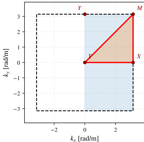
(b) Reciprocal space & symmetry path
