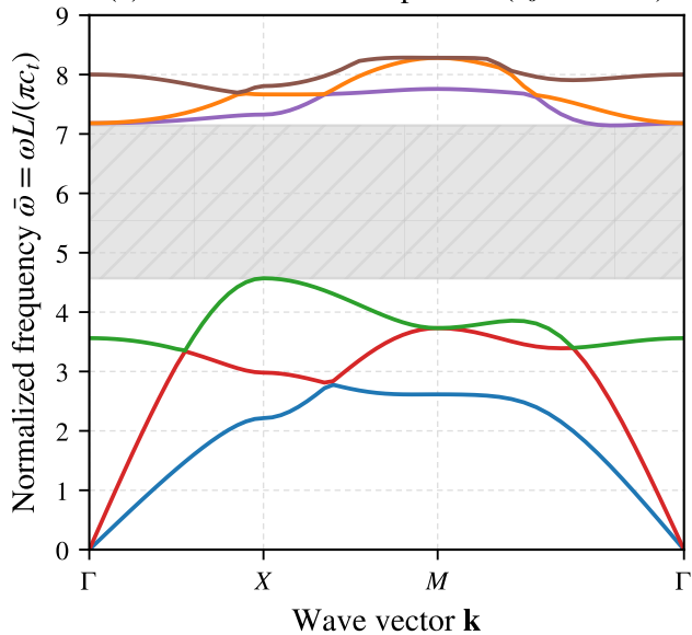
(a) Case C baseline dispersion ( r_0/a = 0.30 )
