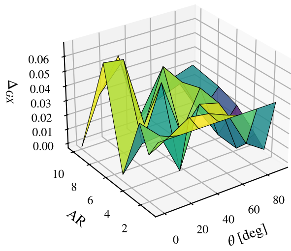
(a) Response surface \Delta_{GX}(\theta, AR)
