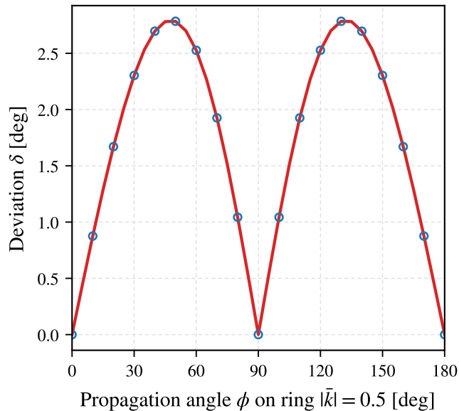
(b) Mirror co-symmetry of \delta(\phi) , AR=10
