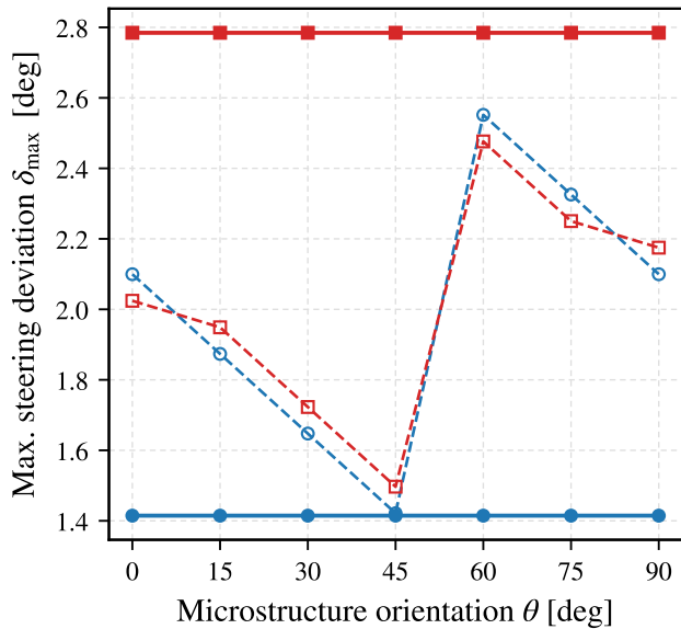
(a) Steering strength & axis vs \theta
