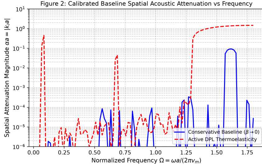
Figure 2: Calibrated baseline spatial acoustic attenuation \alpha a = |k_i a| versus normalized frequency \Omega for Family S1. The conservative baseline exhibits numerical-floor attenuation ( \alpha a \approx 1.67 \times 10^{-5} ) across pass bands, whereas active DPL thermoelasticity establishes an active dissipation baseline ( \alpha a_{\text{mean}} = 2.21 \times 10^{-4} ).
