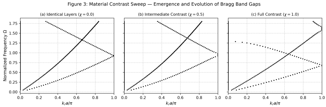
Figure 3: Material contrast sweep (Family S2) showing the emergence and evolution of Bragg band gaps across \chi = 0.0 (identical layers), \chi = 0.5 , and \chi = 1.0 (full contrast).
