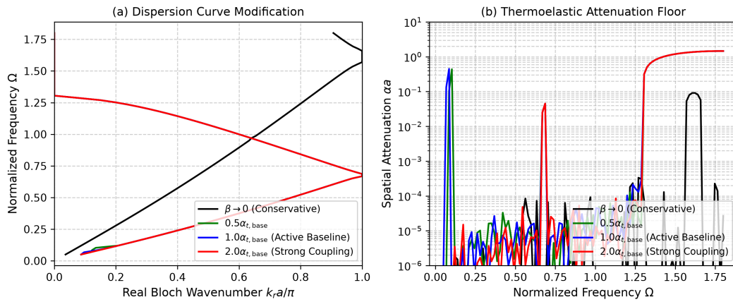
Figure 7: Thermoelastic coupling intensity sensitivity and band-edge blunting (Family S6): (a) acoustic dispersion modification; (b) spatial attenuation floor scaling across \alpha_t/\alpha_{t, \text{base}} \in \{0.0, 0.5, 1.0, 2.0\} .
