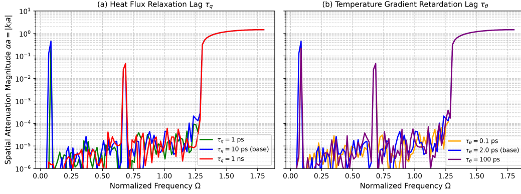
Figure 6: Dual-Phase-Lag (DPL) non-Fourier thermal time lags on continuous acoustic attenuation (Family S5): (a) heat flux relaxation lag \tau_q \in \{1 \text{ ps}, 10 \text{ ps}, 1 \text{ ns}\} ; (b) temperature gradient retardation lag \tau_\theta \in \{0.1 \text{ ps}, 2 \text{ ps}, 100 \text{ ps}\} .
