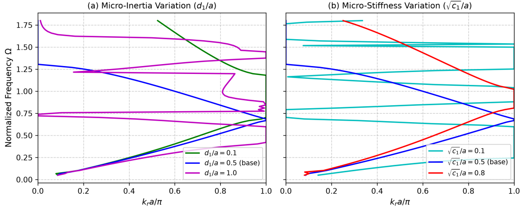
Figure 4: Dipolar gradient-elastic length-scale sensitivity on continuous acoustic dispersion (Family S3): (a) micro-inertia variation d_1/a \in \{0.1, 0.5, 1.0\} ; (b) micro-stiffness variation \sqrt{c_1}/a \in \{0.1, 0.5, 0.8\} .
