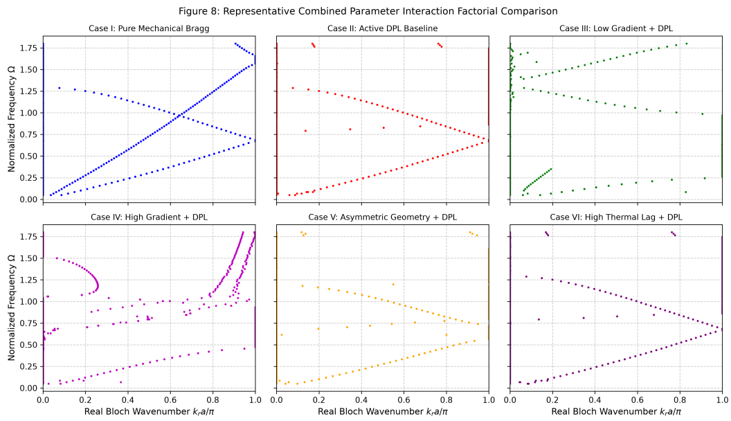
Figure 8: Factorial combined parameter interaction study (Family S7) across six distinct mechanism pairings, confirming the independent physical action of Bragg scattering, gradient elasticity, and DPL thermoelasticity.
