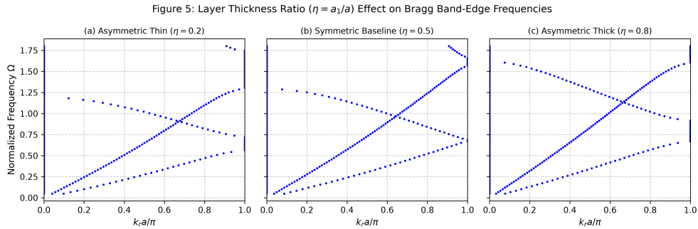
Figure 5: Filling fraction sweep (Family S4) illustrating the effect of layer thickness ratio \eta = a_1/a on band-gap placement and width.
