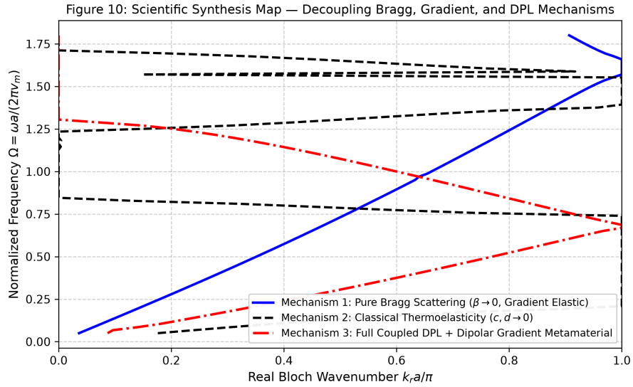
Figure 10: Scientific synthesis map (Family S1 and S3) demonstrating the tripartite decoupling among: (1) Pure Bragg scattering ( \beta \rightarrow 0 , gradient elastic); (2) Classical thermoelasticity ( c, d \rightarrow 0 ); and (3) Full coupled DPL dipolar gradient metamaterial.
