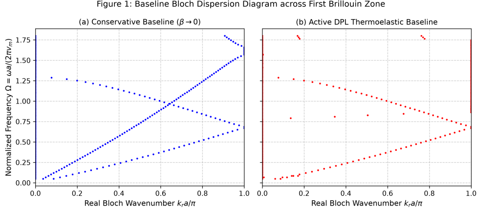
Figure 1: Baseline Bloch dispersion diagram ( \Omega versus k_r a / \pi ) for Family S1, comparing the conservative mechanical baseline ( \beta \rightarrow 0 , blue circles) and the active DPL thermoelastic metamaterial (red crosses). The primary closed Bragg stop band opens at \Omega \in [0.6687, 0.7040] .
