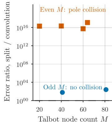
Inversion failure ratio by parity
