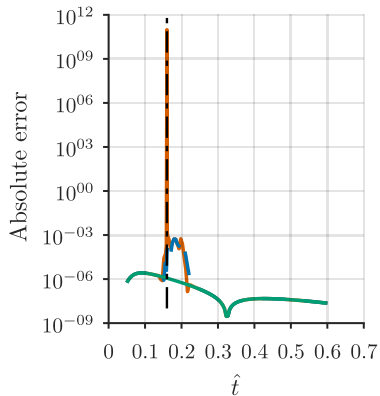
Talbot pole collision in time
