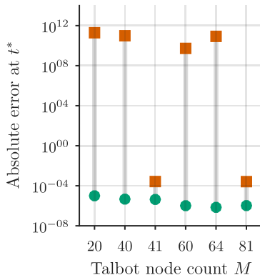
Parity dependence of the inversion
