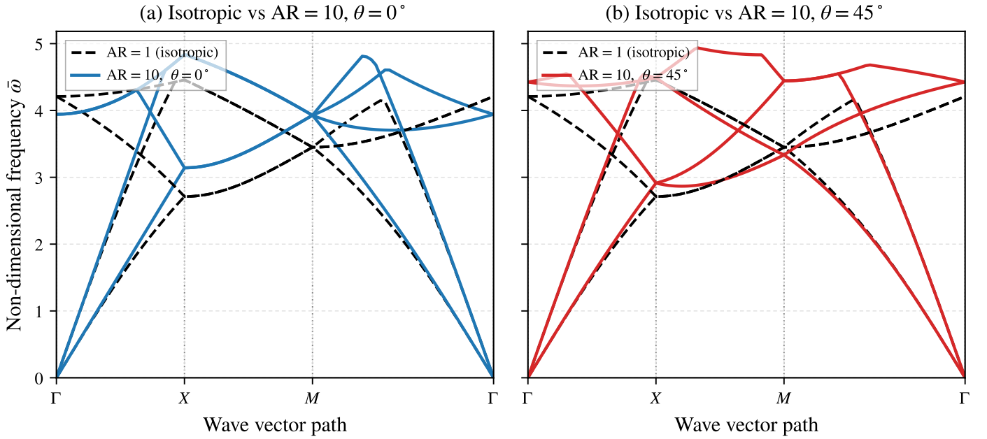
Figure 5: Case-H Bloch bands along \Gamma - X - M - \Gamma . (a) Isotropic reference ( \text{AR} = 1 ) and aligned anisotropy ( \text{AR} = 10, \theta = 0^\circ ). (b) Isotropic reference and diagonal anisotropy ( \text{AR} = 10, \theta = 45^\circ ), which opens a \Gamma - X stop band but no complete gap.
