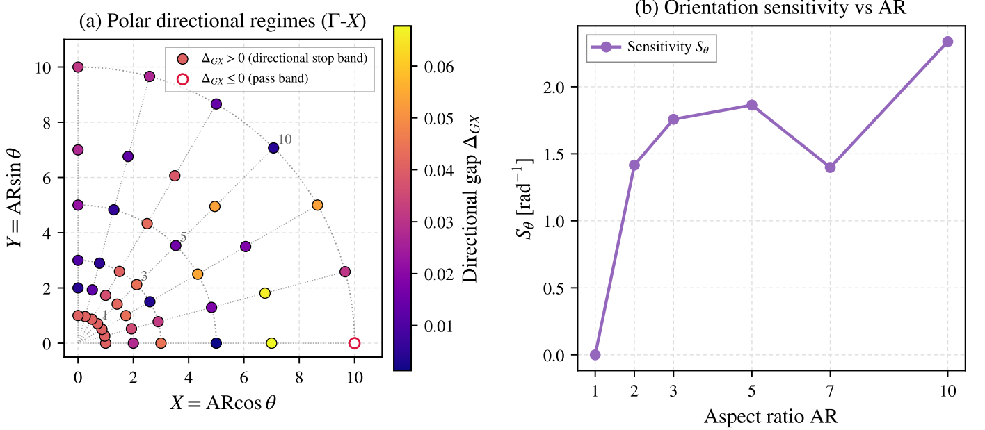
Figure 9: Polar-coordinate view of the sampled Case-H designs, classified by \Delta_{GX} \leq 0 (pass band) and \Delta_{GX} > 0 (directional stop band). The displayed boundary is a visual summary of sampled points.
