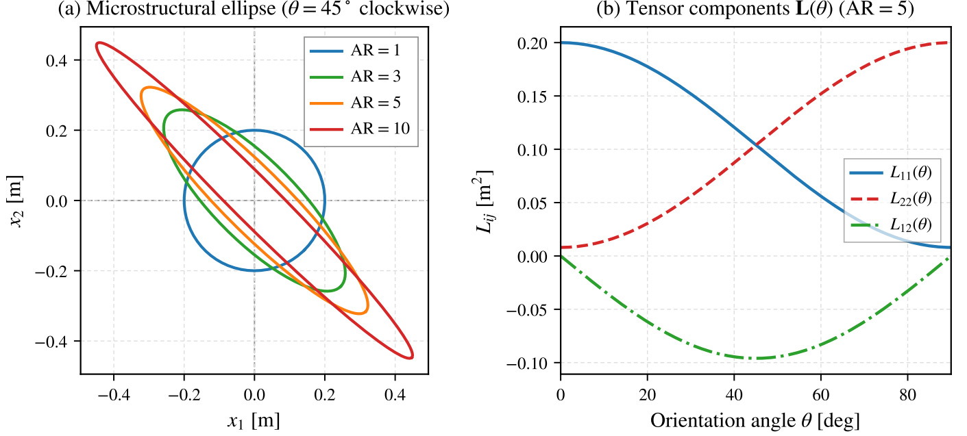
Figure 1: (a) Area-preserving averaging ellipses at \theta = 45^\circ for \text{AR} = 1, 3, 5, 10 , with positive orientation measured clockwise. (b) Length-tensor components versus orientation for \text{AR} = 5 , including L_{12}(45^\circ) = -0.096 \text{ m}^2 under the same passive-rotation convention.
