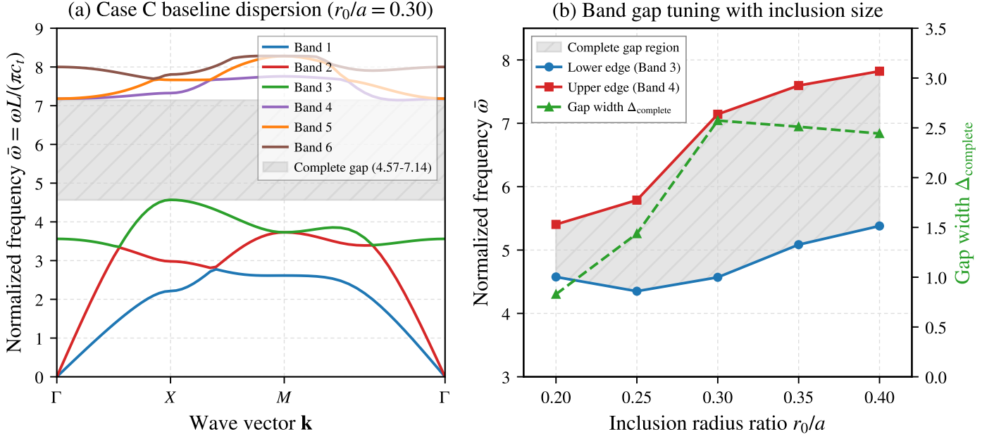
Figure 12: Case-C complete-gap formation and radius dependence. (a) Bands along \Gamma - X - M - \Gamma for r_0/L = 0.30 , with the 4 \times 4 -mesh gap between Bands 3 and 4. (b) Complete-gap width versus r_0/a at the same mesh; the r_0/a = 0.30 result is not mesh-converged.
