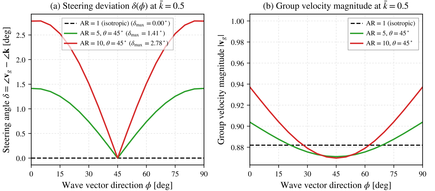
Figure 10: Acoustic-branch group-velocity steering on |\mathbf{k}| = 0.5 at \theta = 45^\circ . (a) Angular deviation for AR = 1, 5, 10, with peak values 0^\circ , 1.4146^\circ , and 2.7846^\circ . (b) Directional variation of group-velocity magnitude.
