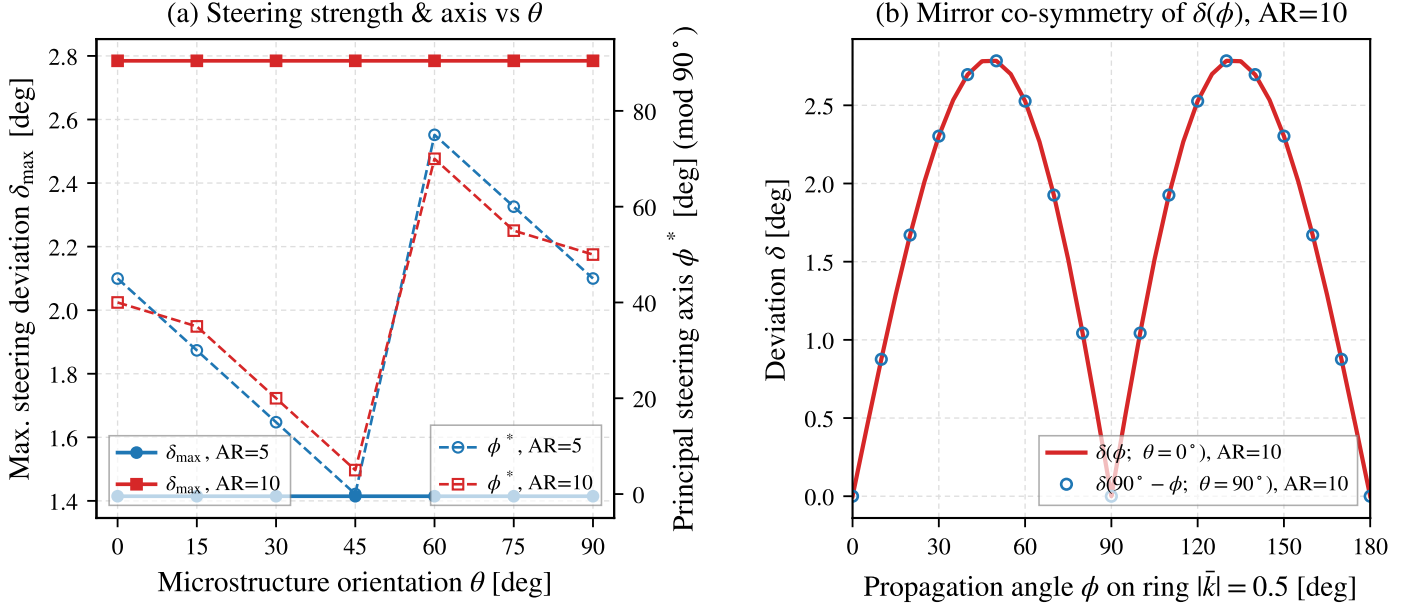
Figure 11: Orientation dependence of steering on |\mathbf{k}| = 0.5 . (a) Peak deviation \delta_{\max} and principal direction \phi^* for AR = 5, 10; the peak amplitude is invariant over the sampled orientations, while the lobe direction follows the rotated tensor axes on the 5° ring grid. (b) The \theta = 0^\circ and 90^\circ deviation fields at AR = 10 exhibit mirror co-symmetry.
