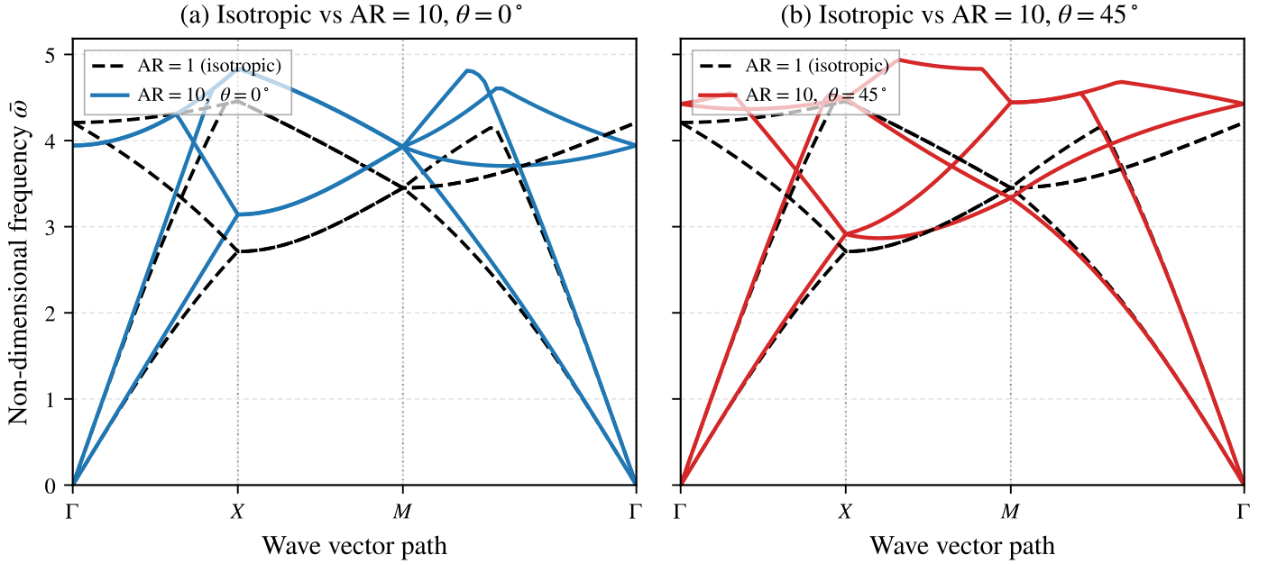
Figure 5: Case-H Bloch bands along \Gamma - X - M - \Gamma . (a) Isotropic reference ( \text{AR} = 1 ) and aligned anisotropy ( \text{AR} = 10 , \theta = 0^\circ ). (b) Isotropic reference and diagonal anisotropy ( \text{AR} = 10 , \theta = 45^\circ ), which opens a \Gamma - X stop band but no complete gap.
