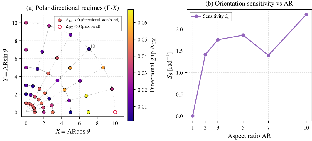
Figure 11: Polar design map ( X = AR \cos \theta, Y = AR \sin \theta ) classifying the elastodynamic response into Pass-Band ( \Delta_{GX} \leq 0 ) and Directional Stop-Band ( \Delta_{GX} > 0 ) regimes. Verified simulation points and empirical regime boundaries are shown.
