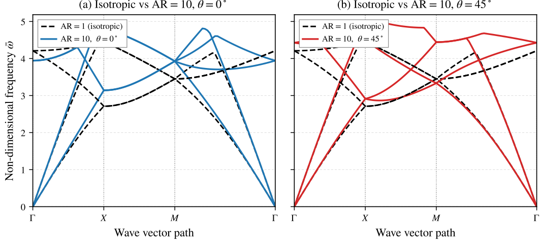
Figure 6: Bloch band structure along \Gamma-X-M-\Gamma for Case H ( L = 1.0 m, \rho = 1.0 kg/m 3 , \mu = 1.0 Pa, \nu = 0.25 , l_{\text{iso}} = 0.20 m, \ell_i = 0.20 m). (a) Isotropic baseline ( AR = 1 ) versus anisotropic microstructure aligned with the lattice ( AR = 10, \theta = 0^\circ ). (b) Isotropic baseline ( AR = 1 ) versus diagonal anisotropic microstructure ( AR = 10, \theta = 45^\circ ), highlighting the opening of directional stop band \Delta_{GX} = +0.0043 along \Gamma-X while strictly preserving the absence of complete omnidirectional band gaps ( \Delta_{\text{complete}} \leq -0.3235 ).
