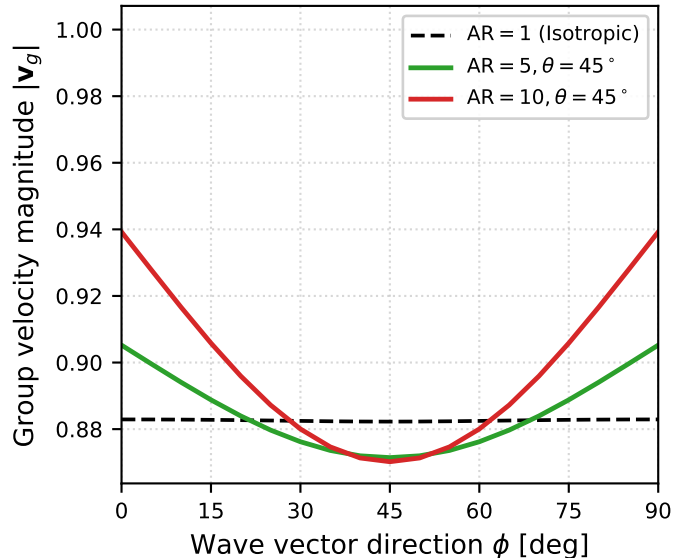
(b) Group Velocity Magnitude at \bar{k} = 0.5
