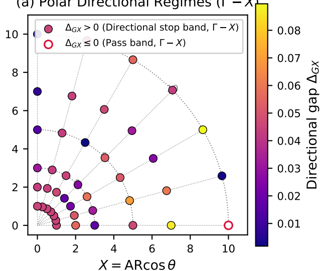
(a) Polar Directional Regimes ( \Gamma - X )
