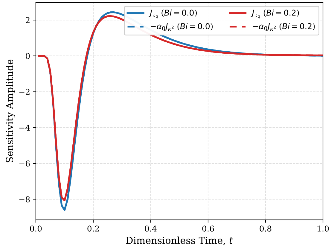
(a) Exact Sensitivity Collinearity: J_{\tau_q}(t) \equiv -\alpha_0 J_{\kappa^2}(t)
