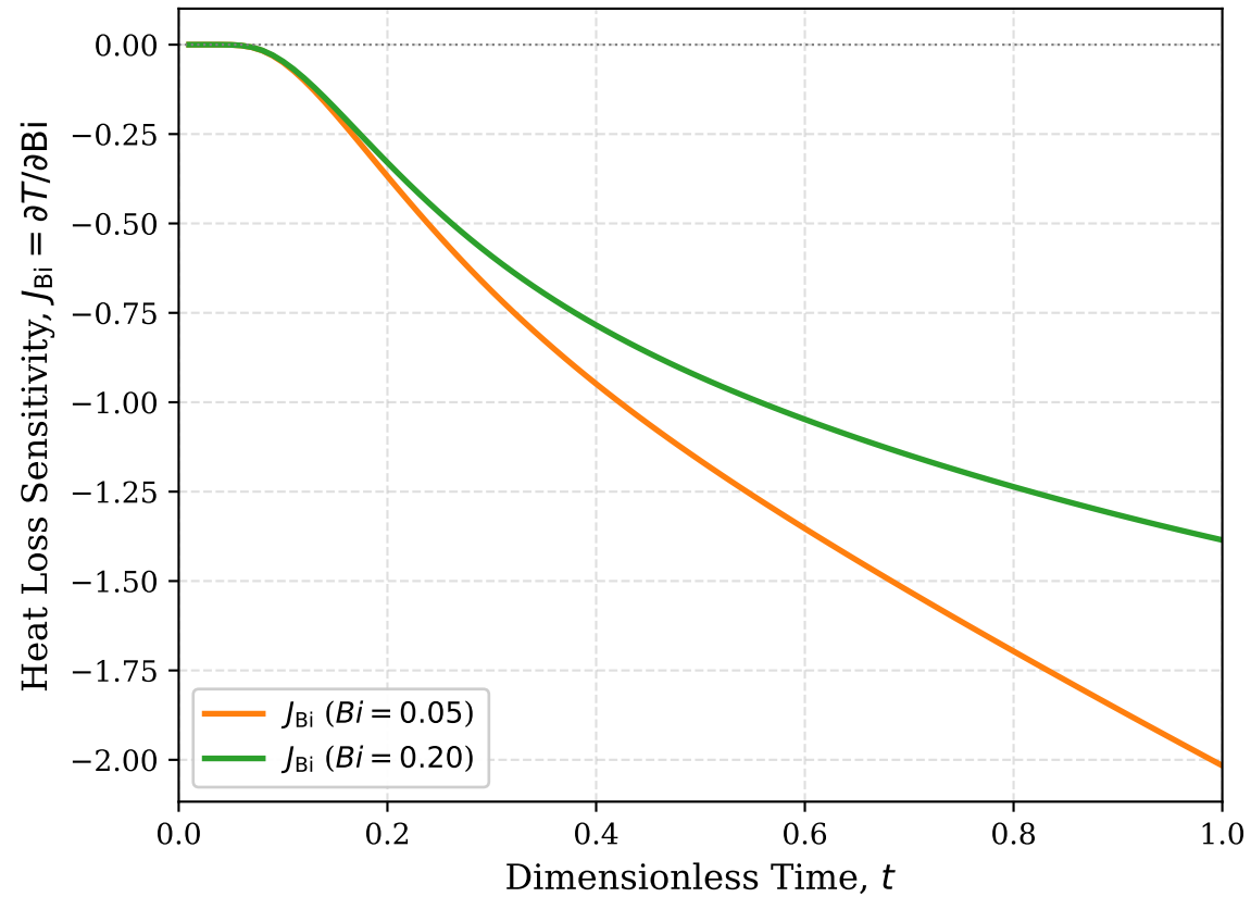
(b) Independent Cooling Tail Sensitivity Profile
