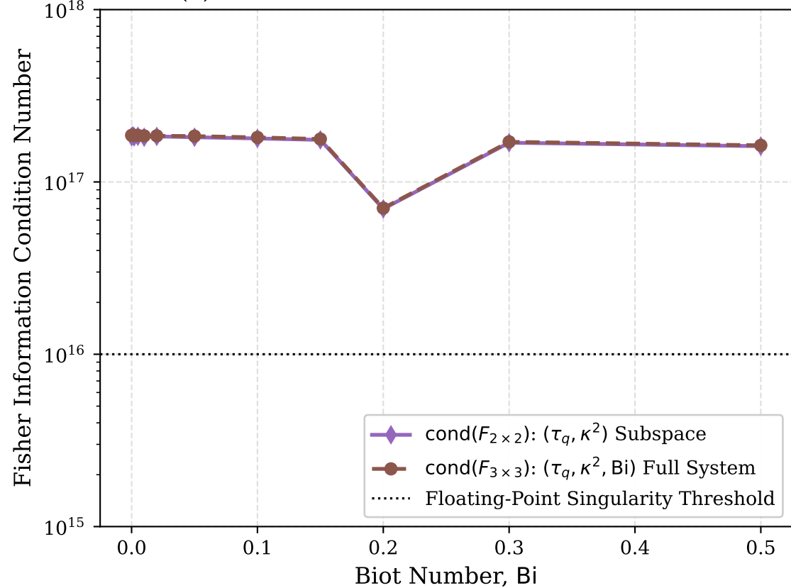
(b) Fisher Condition Numbers vs Biot Number
