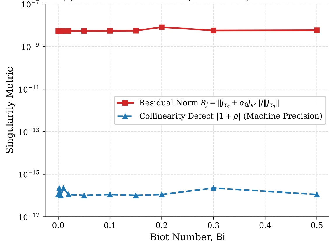
(a) Invariance of Sensitivity Collinearity to Heat Loss
