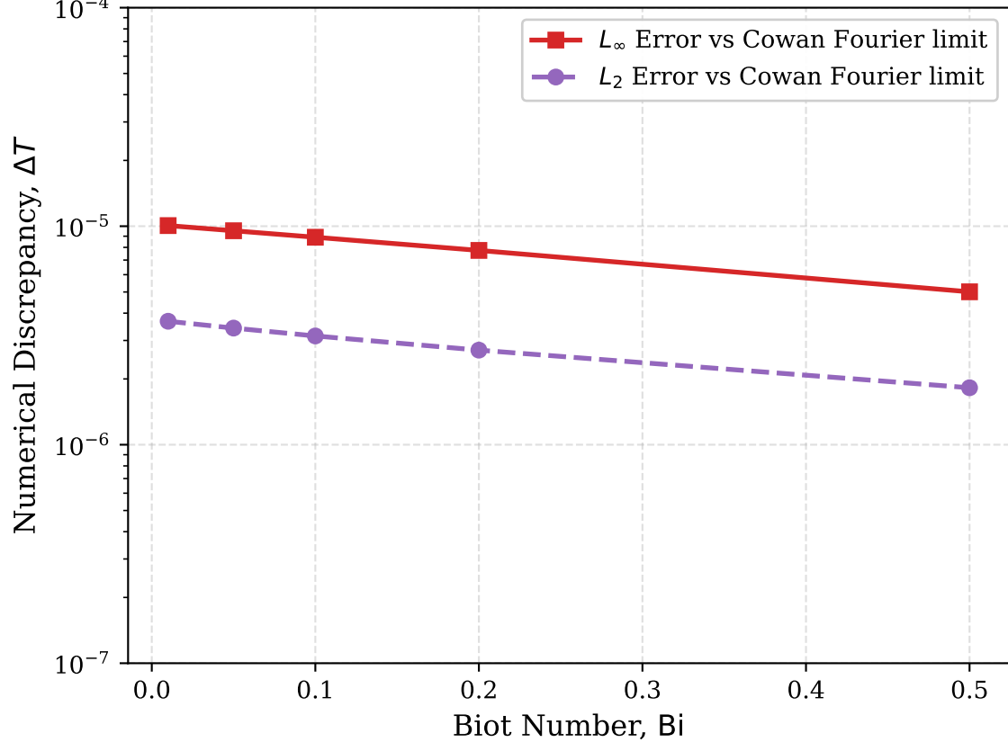
(b) Absolute Identity with Cowan (1963) Fourier Solution
