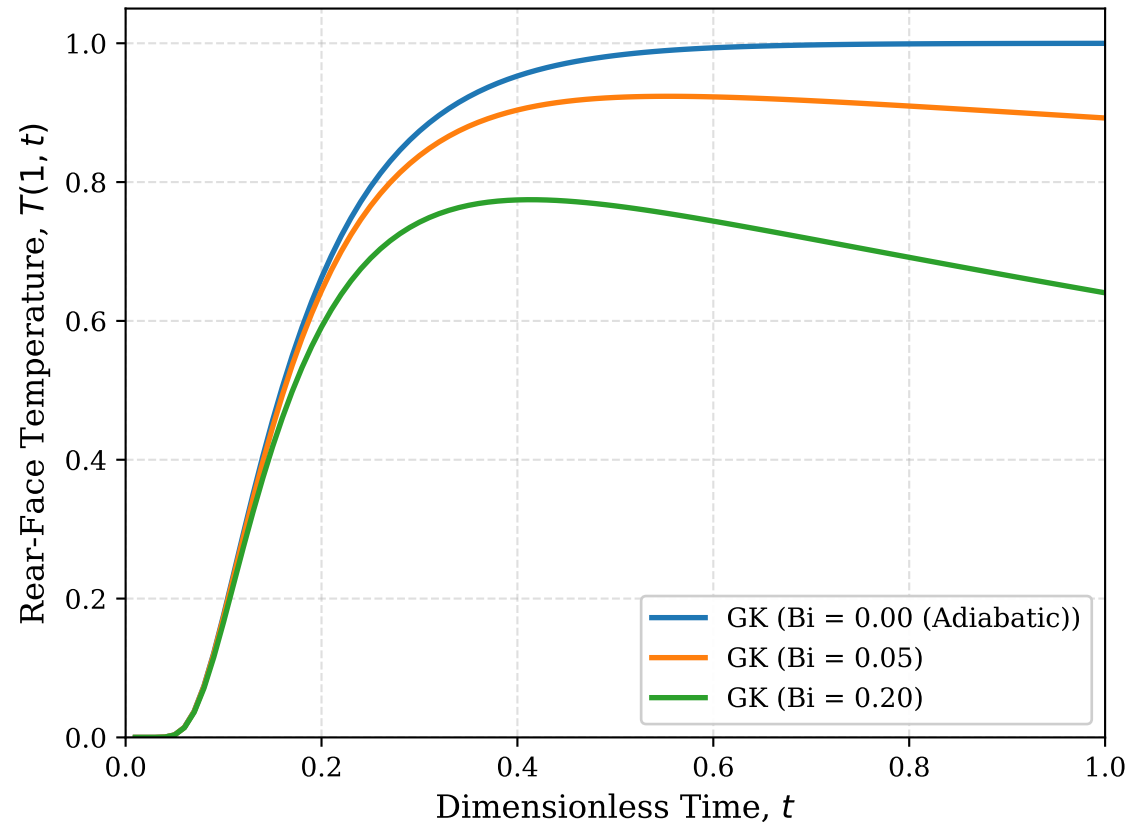
(a) Rear-Face Thermal Response across Biot Numbers
