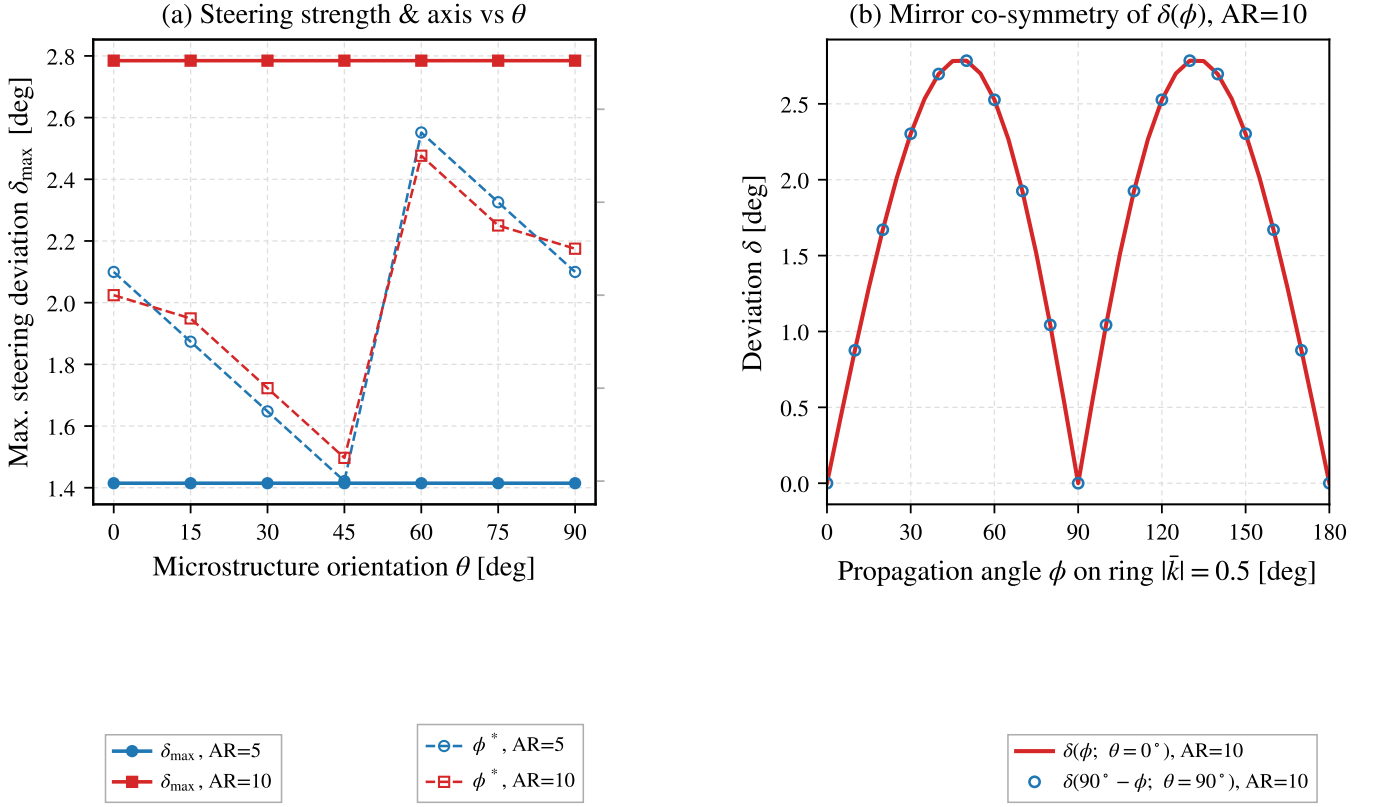
Figure 12: Orientation dependence of steering on |\mathbf{k}| = 0.5 . (a) Peak deviation \delta_{\max} and principal direction \phi^* for \text{AR} = 5, 10 ; the peak angular deviation is invariant over the sampled orientations, while the lobe direction follows the rotated tensor axes on the 5^\circ ring grid. (b) The \theta = 0^\circ and 90^\circ deviation fields at \text{AR} = 10 exhibit mirror co-symmetry.
