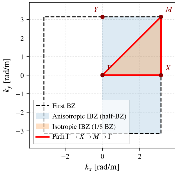
(b) Reciprocal space &amp; symmetry path
