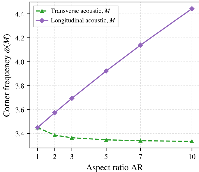
(b) Frequencies at M
