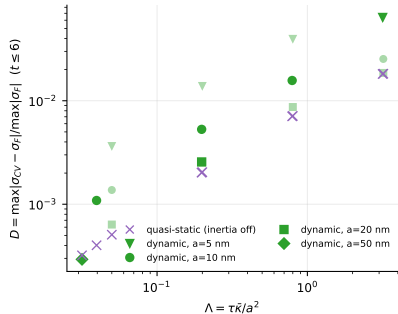
(a) thermal-memory deviation of the wall hoop stress
