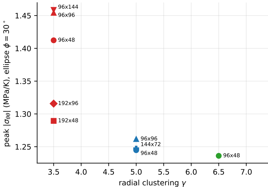
near-wall clustering controls the tip stress
