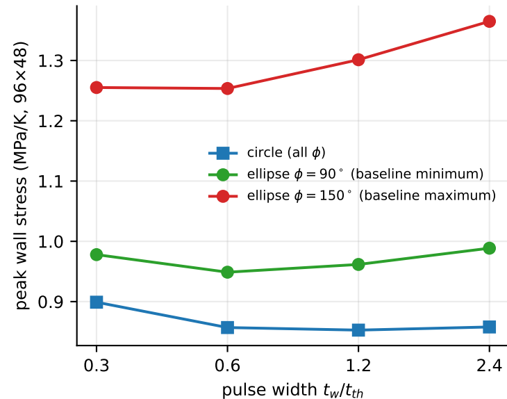
(a) peak stress versus pulse width
