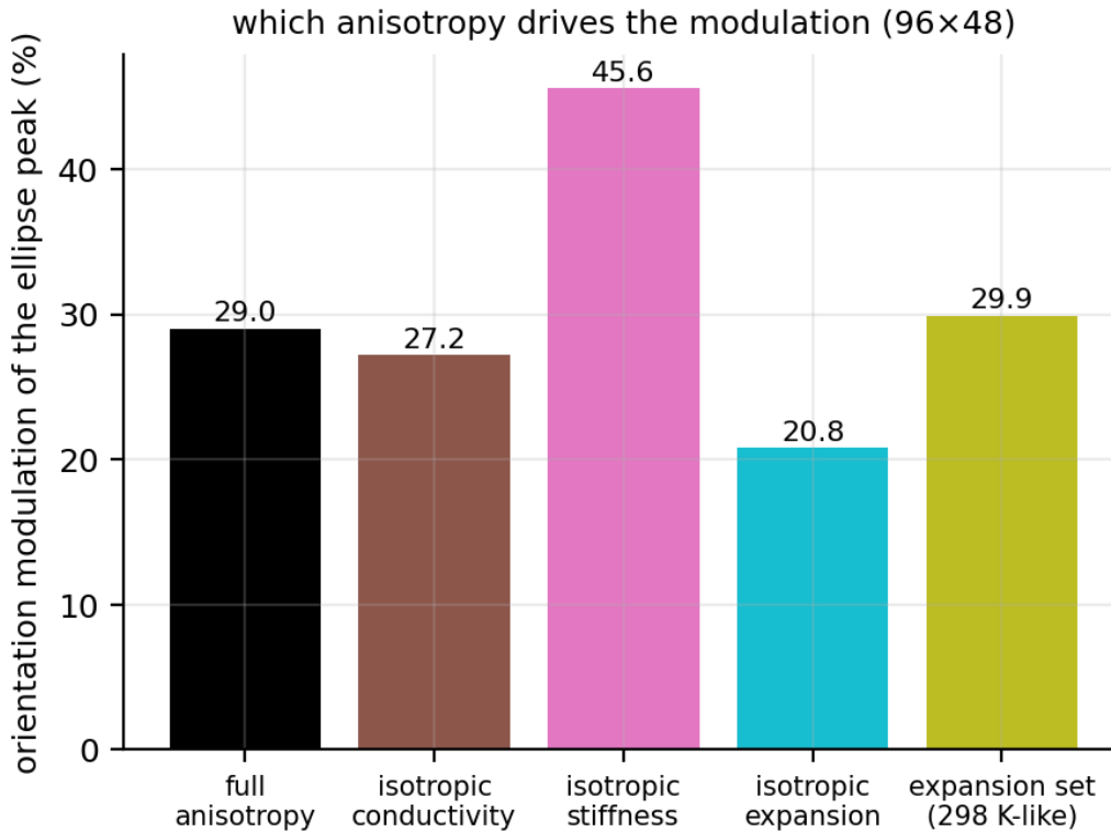
Fig. 7. Orientation modulation of the ellipse peak stress for the baseline and with one anisotropic tensor made isotropic, and for the 298 K-like expansion set ( 96 \times 48 , six orientations).
