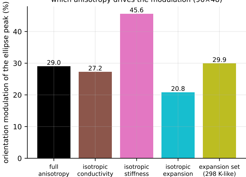
which anisotropy drives the modulation (96×48)
