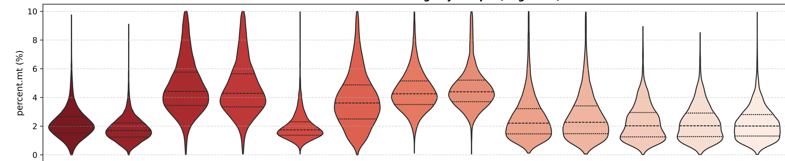
Mitochondrial Read Percentage by Sample (orig.ident)
