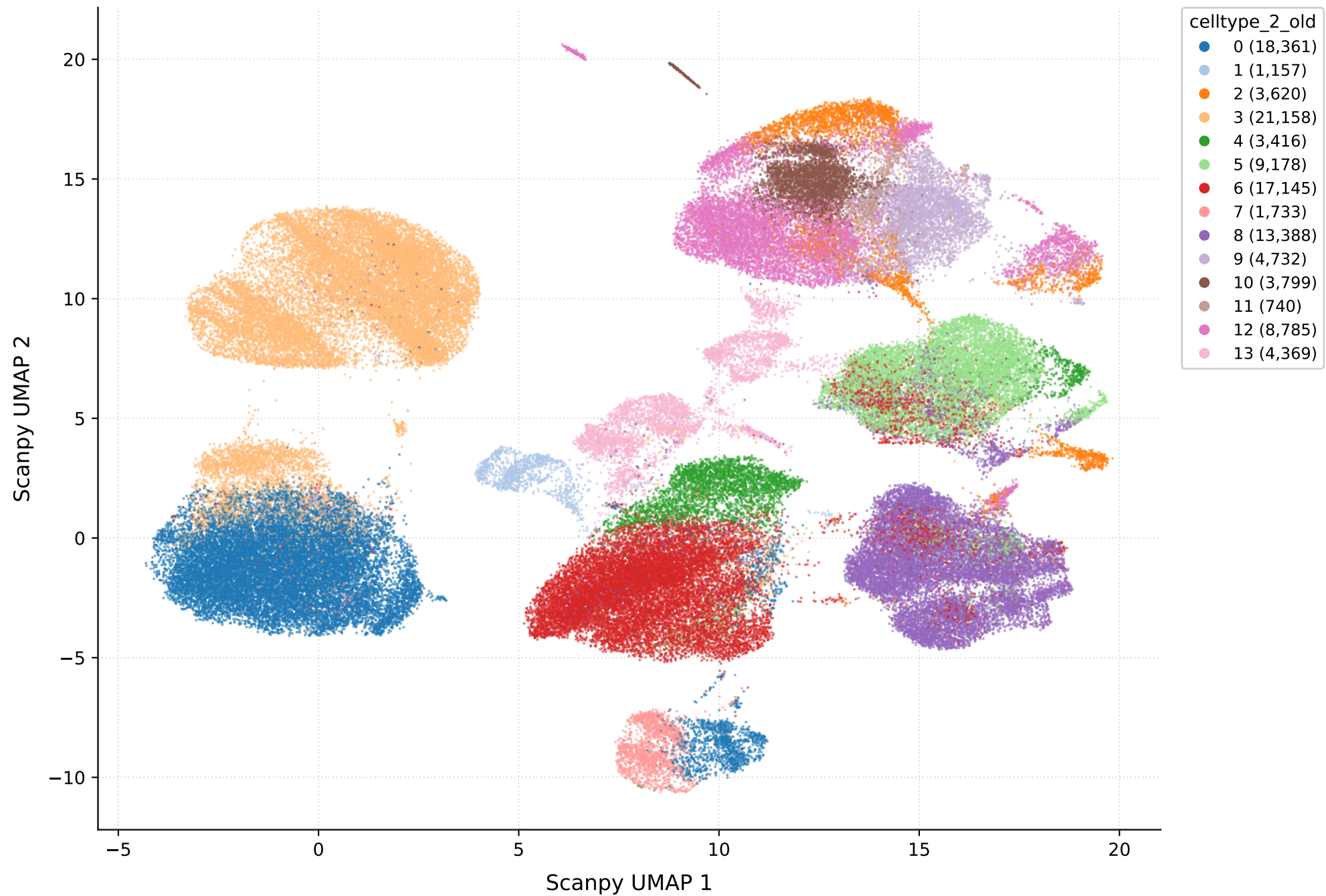
Scanpy UMAP: celltype_2_old (n = 111,581 cells, 14 groups)
